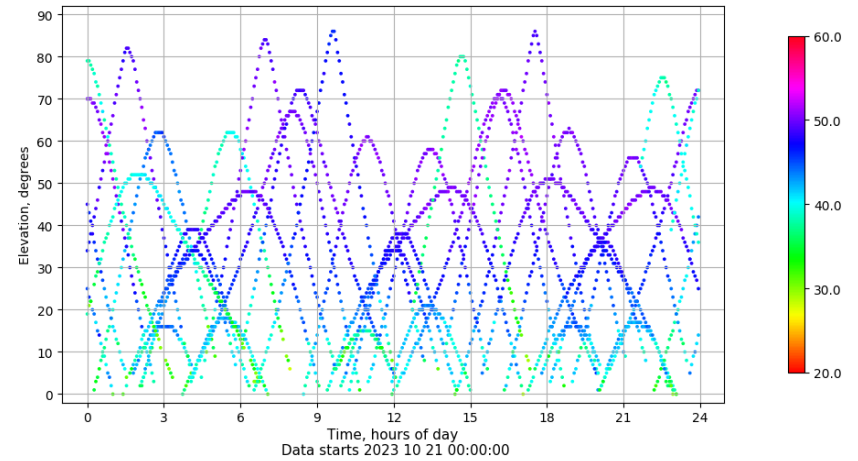
Time-elevation plot for station LP01. Signal to Noise S1C Data file LP0100ESP_R_2023294.xtr
