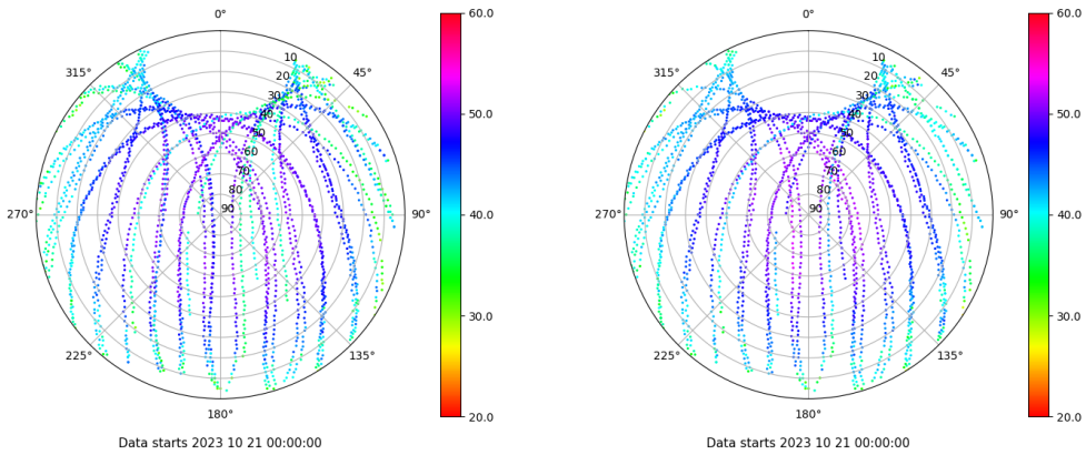
Skyplot for station LP01. Signal to Noise S1C Data file LP0100ESP_R_2023294.xtr Skyplot for station LP01. Signal to Noise S2C Data file LP0100ESP_R_2023294.xtr
