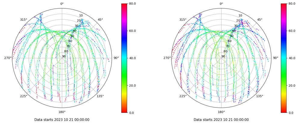
Skyplot for station LP01. Parameter M1C Data file LP0100ESP_R_2023294.xtr Skyplot for station LP01. Parameter M2C Data file LP0100ESP_R_2023294.xtr
