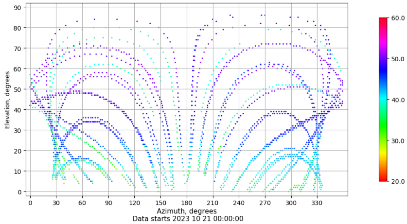
Azimuth-elevation plot for station LP01. Signal to Noise S1C Data file LP0100ESP_R_2023294.xtr
