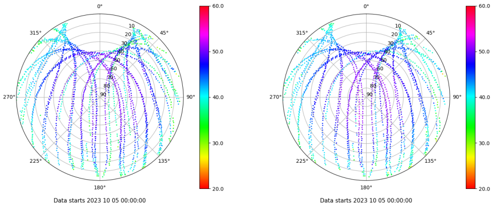
Skyplot for station LP01. Signal to Noise S1C Data file LP0100ESP_R_2023278.xtr Skyplot for station LP01. Signal to Noise S2C Data file LP0100ESP_R_2023278.xtr
