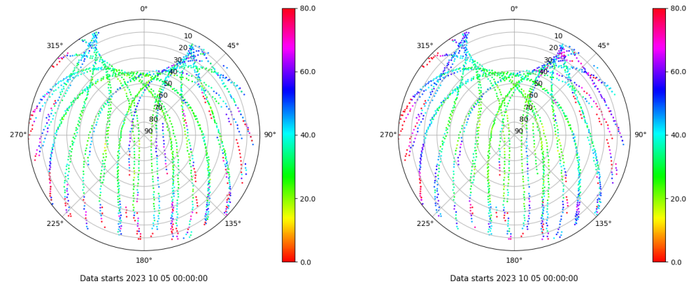
Skyplot for station LP01. Parameter M1C Data file LP0100ESP_R_2023278.xtr Skyplot for station LP01. Parameter M2C Data file LP0100ESP_R_2023278.xtr
