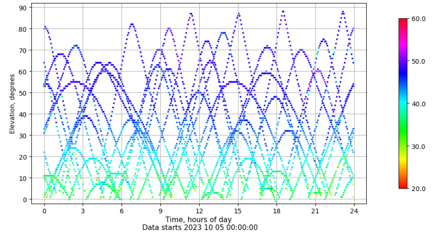
Time-elevation plot for station LP01. Signal to Noise S1C Data file LP0100ESP_R_2023278.xtr
