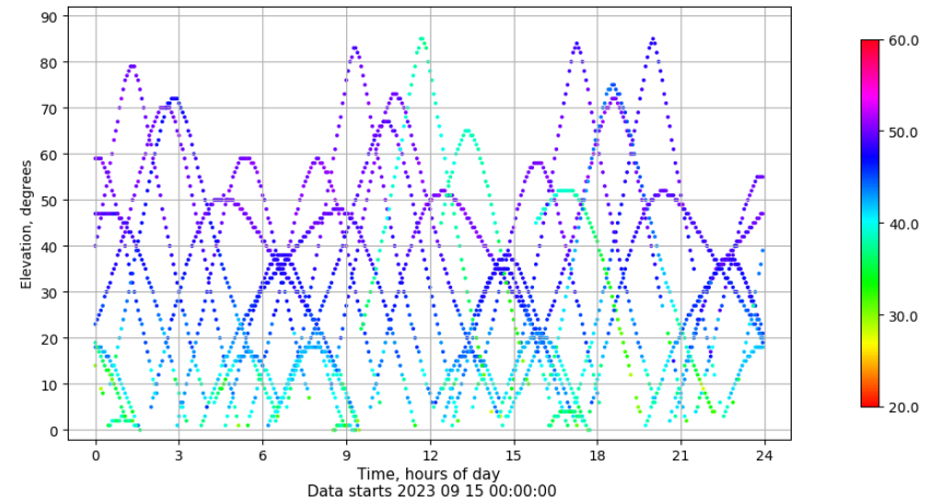
Time-elevation plot for station LP01. Signal to Noise S1C Data file LP0100ESP_R_2023258.xtr
