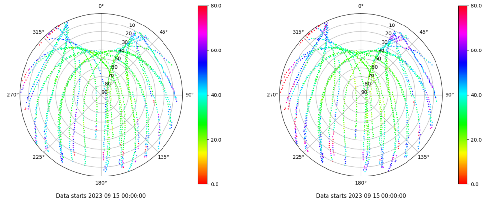
Skyplot for station LP01. Parameter M1C Data file LP0100ESP_R_2023258.xtr Skyplot for station LP01. Parameter M2C Data file LP0100ESP_R_2023258.xtr
