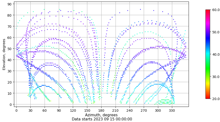
Azimuth-elevation plot for station LP01. Signal to Noise S1C Data file LP0100ESP_R_2023258.xtr
