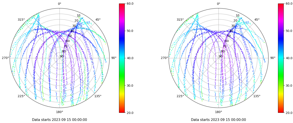
Skyplot for station LP01. Signal to Noise S1C Data file LP0100ESP_R_2023258.xtr Skyplot for station LP01. Signal to Noise S2C Data file LP0100ESP_R_2023258.xtr
