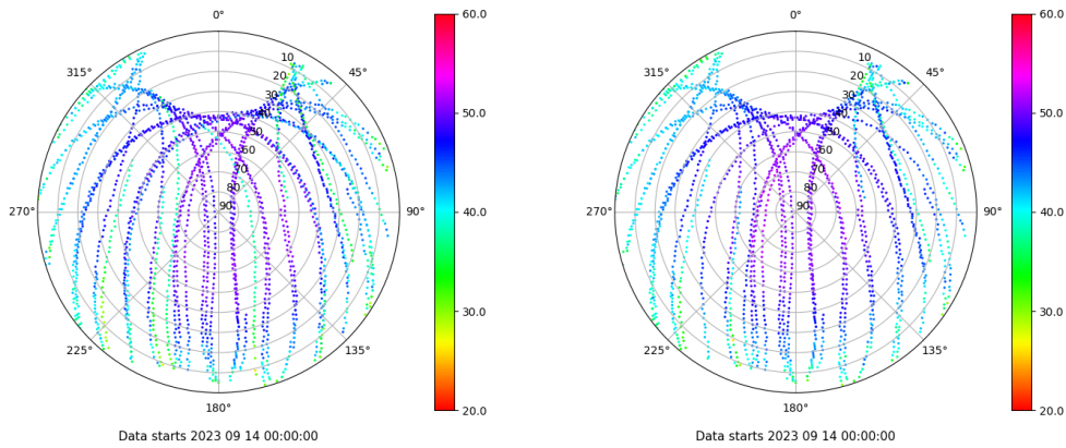
Skyplot for station LP01. Signal to Noise S1C Data file LP0100ESP_R_2023257.xtr Skyplot for station LP01. Signal to Noise S2C Data file LP0100ESP_R_2023257.xtr
