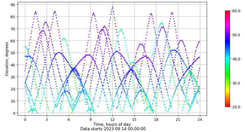
Time-elevation plot for station LP01. Signal to Noise S1C Data file LP0100ESP_R_2023257.xtr
