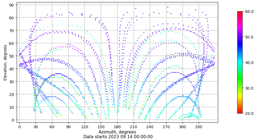
Azimuth-elevation plot for station LP01. Signal to Noise S1C Data file LP0100ESP_R_2023257.xtr
