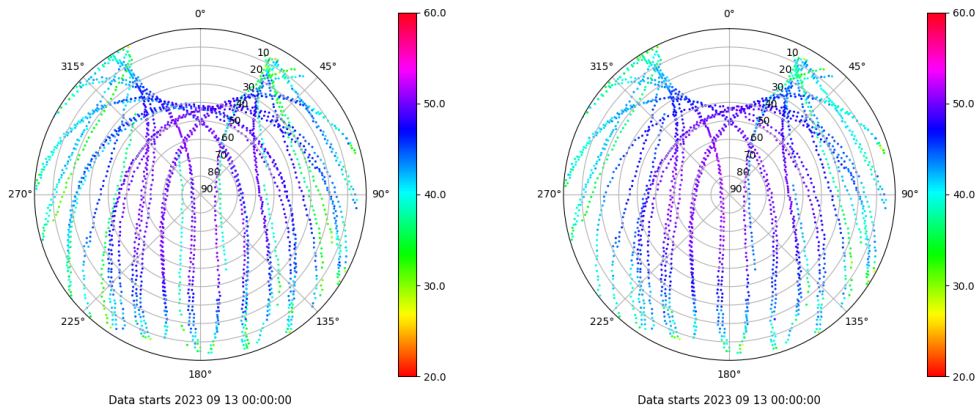
Skyplot for station LP01. Signal to Noise S1C Data file LP0100ESP_R_2023256.xtr Skyplot for station LP01. Signal to Noise S2C Data file LP0100ESP_R_2023256.xtr
