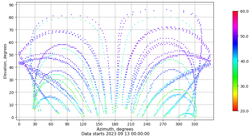
Azimuth-elevation plot for station LP01. Signal to Noise S1C Data file LP0100ESP_R_2023256.xtr
