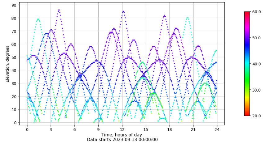
Time-elevation plot for station LP01. Signal to Noise S1C Data file LP0100ESP_R_2023256.xtr
