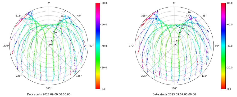
Skyplot for station LP01. Parameter M1C Data file LP0100ESP_R_2023252.xtr Skyplot for station LP01. Parameter M2C Data file LP0100ESP_R_2023252.xtr
