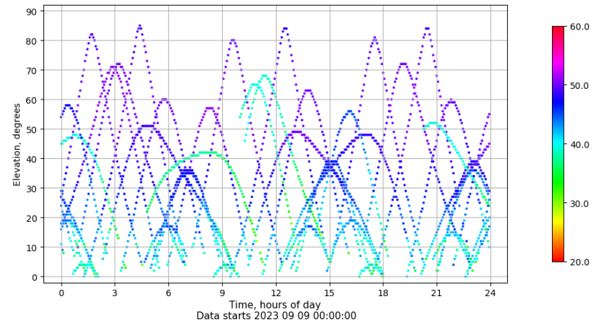
Time-elevation plot for station LP01. Signal to Noise S1C Data file LP0100ESP_R_2023252.xtr
