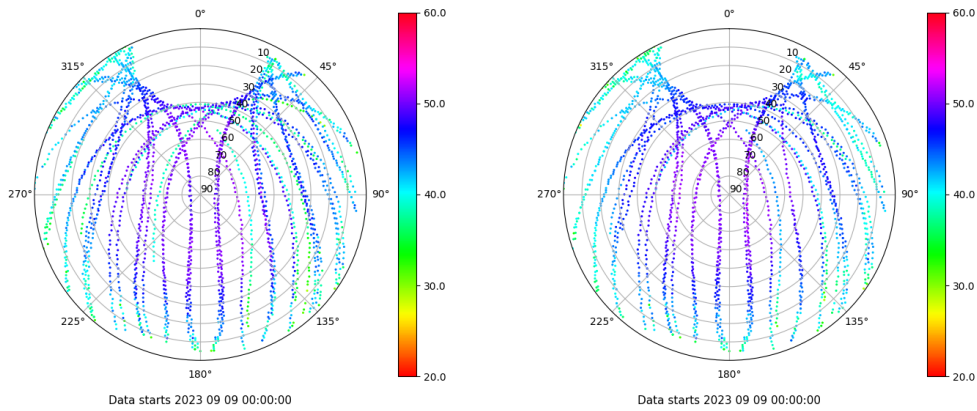
Skyplot for station LP01. Signal to Noise S1C Data file LP0100ESP_R_2023252.xtr Skyplot for station LP01. Signal to Noise S2C Data file LP0100ESP_R_2023252.xtr
