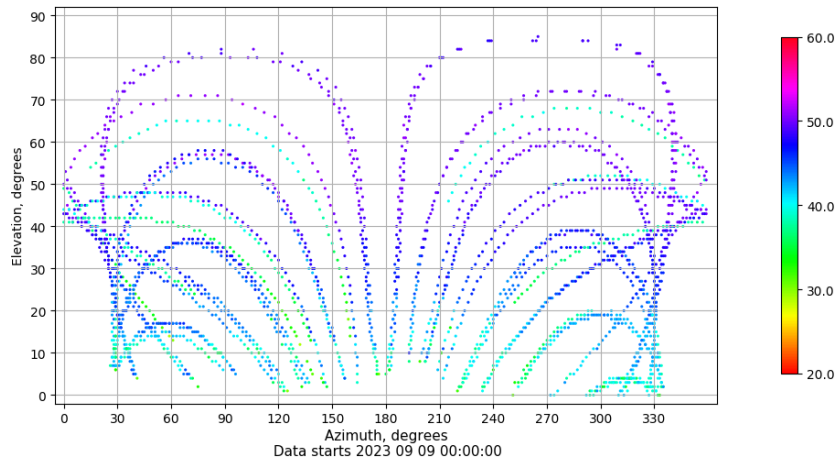
Azimuth-elevation plot for station LP01. Signal to Noise S1C Data file LP0100ESP_R_2023252.xtr
