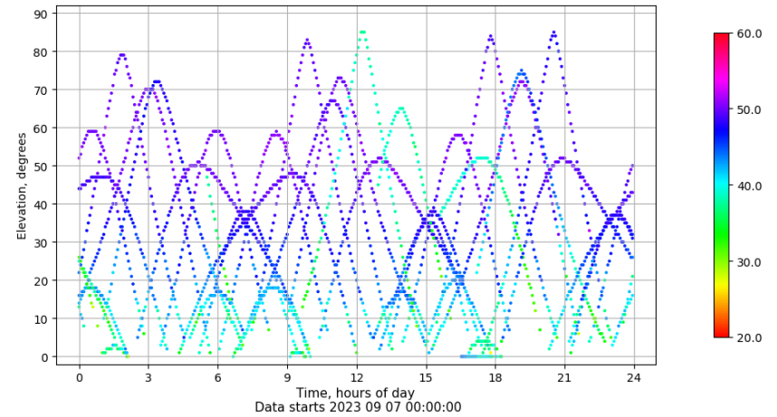
Time-elevation plot for station LP01. Signal to Noise S1C Data file LP0100ESP_R_2023250.xtr
