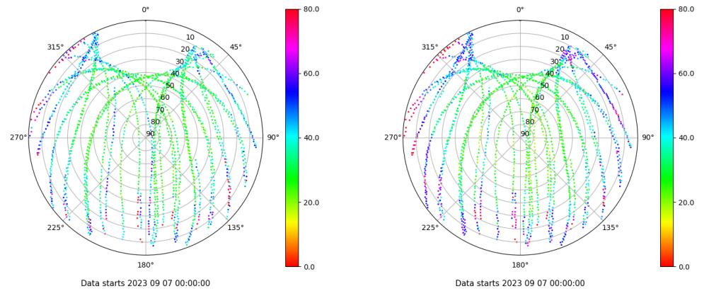
Skyplot for station LP01. Parameter M1C Data file LP0100ESP_R_2023250.xtr Skyplot for station LP01. Parameter M2C Data file LP0100ESP_R_2023250.xtr
