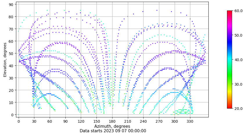
Azimuth-elevation plot for station LP01. Signal to Noise S1C Data file LP0100ESP_R_2023250.xtr
