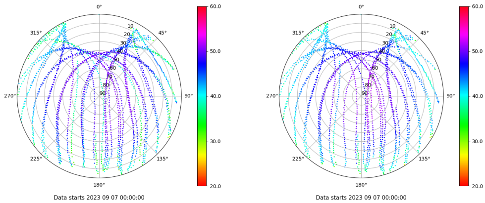
Skyplot for station LP01. Signal to Noise S1C Data file LP0100ESP_R_2023250.xtr Skyplot for station LP01. Signal to Noise S2C Data file LP0100ESP_R_2023250.xtr
