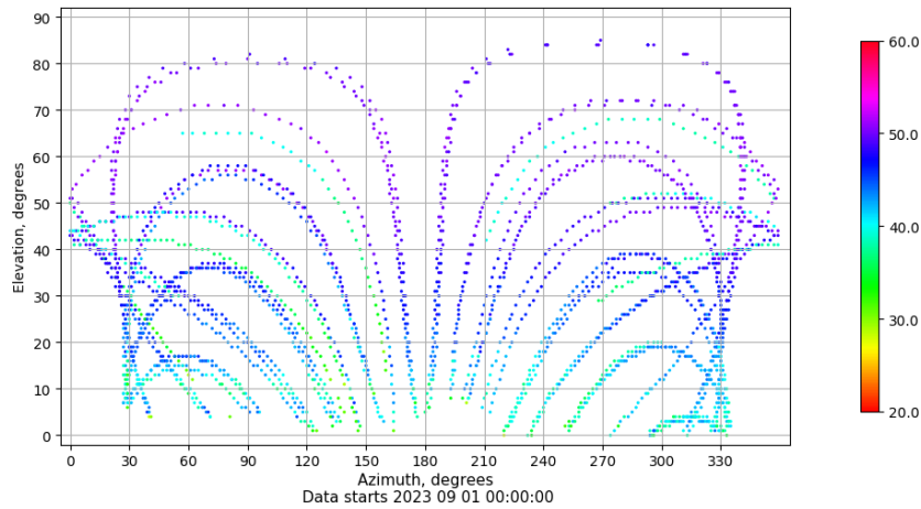
Azimuth-elevation plot for station LP01. Signal to Noise S1C Data file LP0100ESP_R_2023244.xtr
