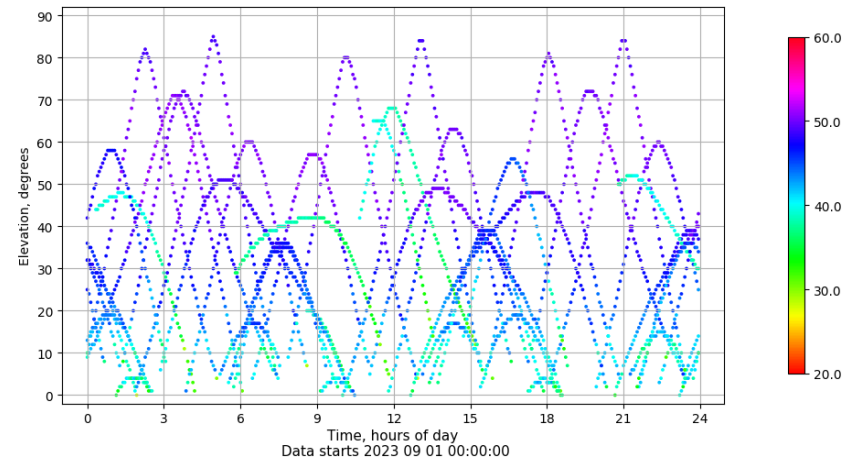
Time-elevation plot for station LP01. Signal to Noise S1C Data file LP0100ESP_R_2023244.xtr
