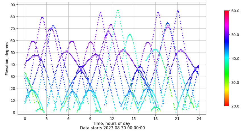
Time-elevation plot for station LP01. Signal to Noise S1C Data file LP0100ESP_R_2023242.xtr
