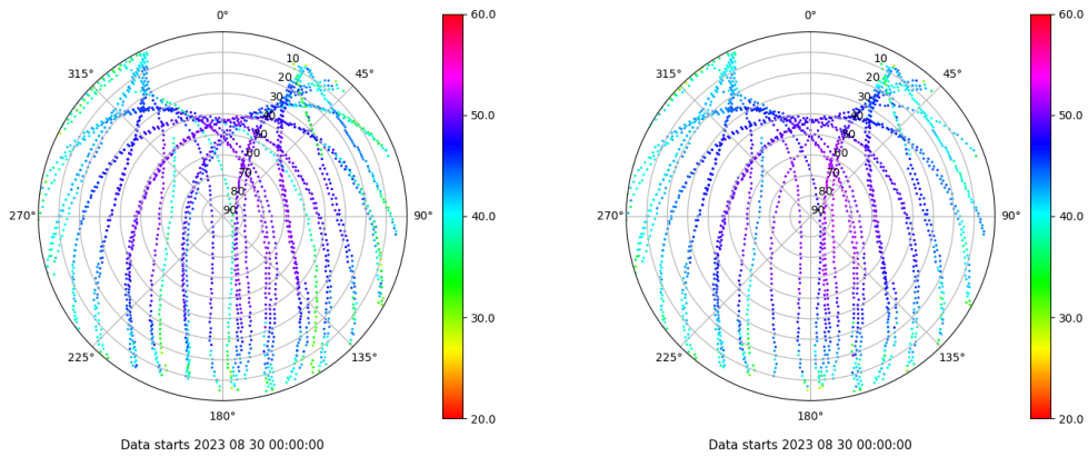
Skyplot for station LP01. Signal to Noise S1C Data file LP0100ESP_R_2023242.xtr Skyplot for station LP01. Signal to Noise S2C Data file LP0100ESP_R_2023242.xtr
