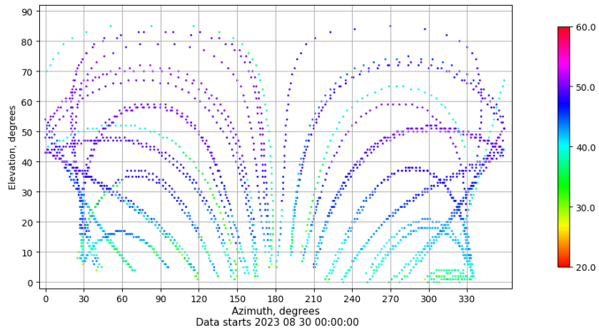
Azimuth-elevation plot for station LP01. Signal to Noise S1C Data file LP0100ESP_R_2023242.xtr
