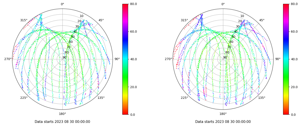
Skyplot for station LP01. Parameter M1C Data file LP0100ESP_R_2023242.xtr Skyplot for station LP01. Parameter M2C Data file LP0100ESP_R_2023242.xtr
