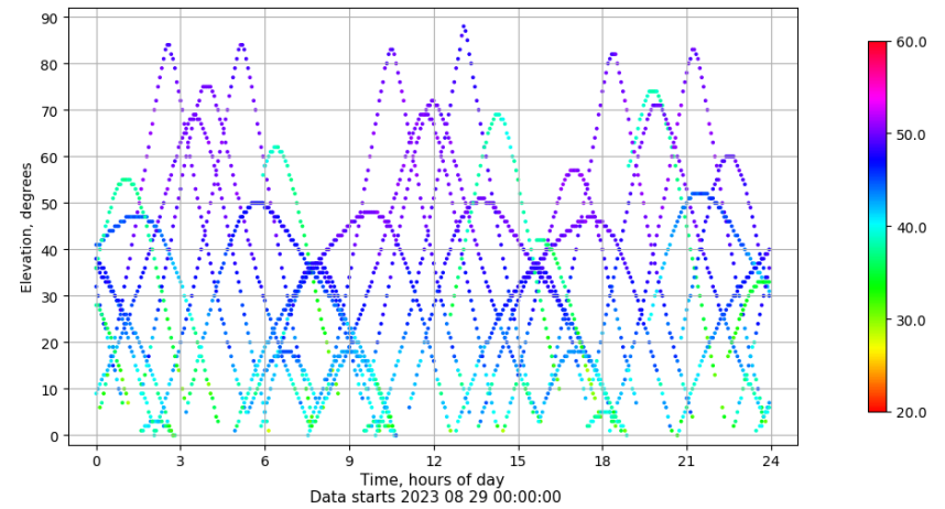
Time-elevation plot for station LP01. Signal to Noise S1C Data file LP0100ESP_R_2023241.xtr
