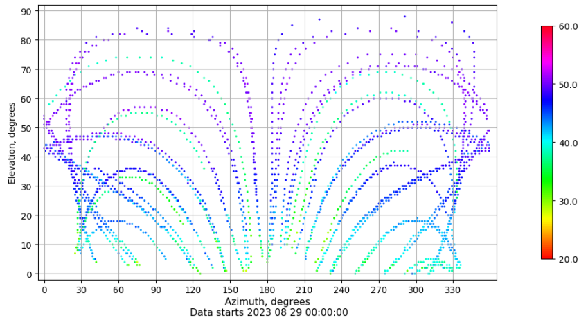
Azimuth-elevation plot for station LP01. Signal to Noise S1C Data file LP0100ESP_R_2023241.xtr
