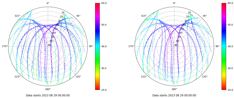
Skyplot for station LP01. Signal to Noise S1C Data file LP0100ESP_R_2023241.xtr Skyplot for station LP01. Signal to Noise S2C Data file LP0100ESP_R_2023241.xtr
