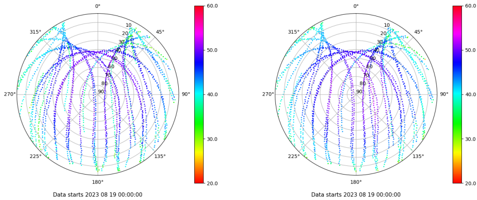
Skyplot for station LP01. Signal to Noise S1C Data file LP0100ESP_R_2023231.xtr Skyplot for station LP01. Signal to Noise S2C Data file LP0100ESP_R_2023231.xtr
