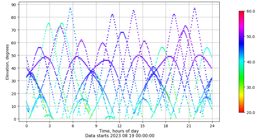
Time-elevation plot for station LP01. Signal to Noise S1C Data file LP0100ESP_R_2023231.xtr
