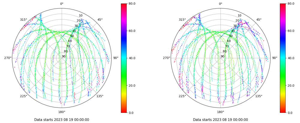
Skyplot for station LP01. Parameter M1C Data file LP0100ESP_R_2023231.xtr Skyplot for station LP01. Parameter M2C Data file LP0100ESP_R_2023231.xtr
