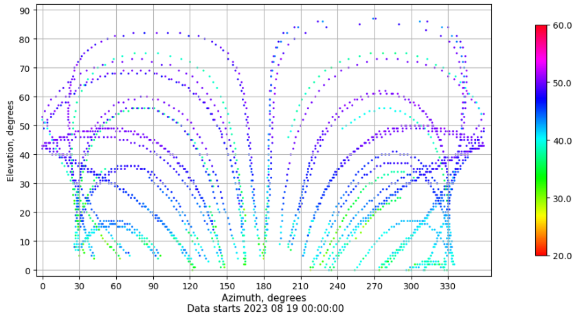
Azimuth-elevation plot for station LP01. Signal to Noise S1C Data file LP0100ESP_R_2023231.xtr
