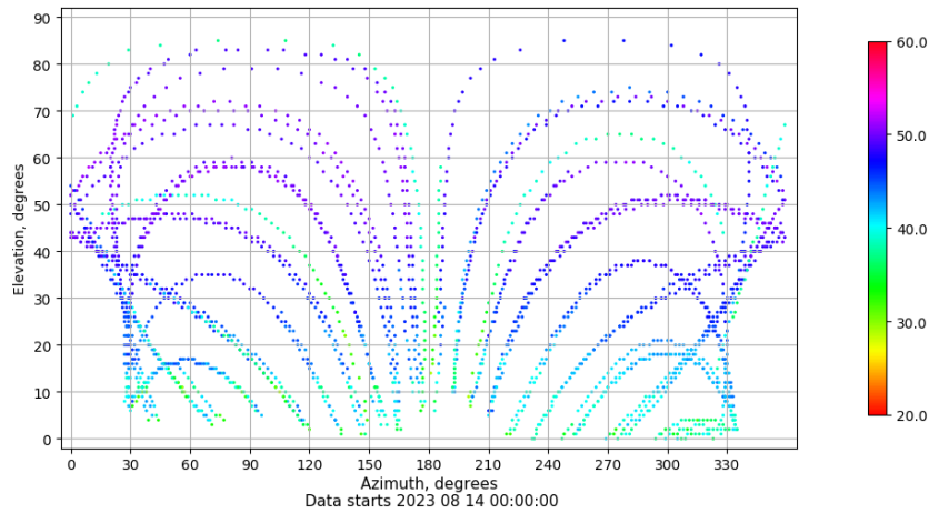
Azimuth-elevation plot for station LP01. Signal to Noise S1C Data file LP0100ESP_R_2023226.xtr
