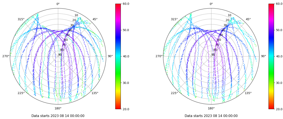
Skyplot for station LP01. Signal to Noise S1C Data file LP0100ESP_R_2023226.xtr Skyplot for station LP01. Signal to Noise S2C Data file LP0100ESP_R_2023226.xtr
