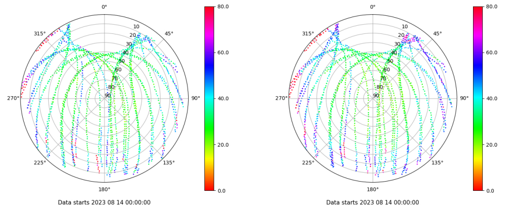
Skyplot for station LP01. Parameter M1C Data file LP0100ESP_R_2023226.xtr Skyplot for station LP01. Parameter M2C Data file LP0100ESP_R_2023226.xtr
