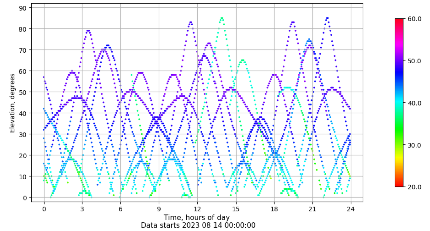
Time-elevation plot for station LP01. Signal to Noise S1C Data file LP0100ESP_R_2023226.xtr
