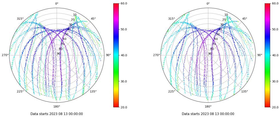
Skyplot for station LP01. Signal to Noise S1C Data file LP0100ESP_R_2023225.xtr Skyplot for station LP01. Signal to Noise S2C Data file LP0100ESP_R_2023225.xtr
