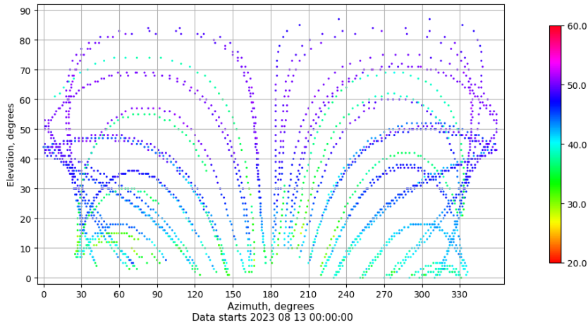
Azimuth-elevation plot for station LP01. Signal to Noise S1C Data file LP0100ESP_R_2023225.xtr
