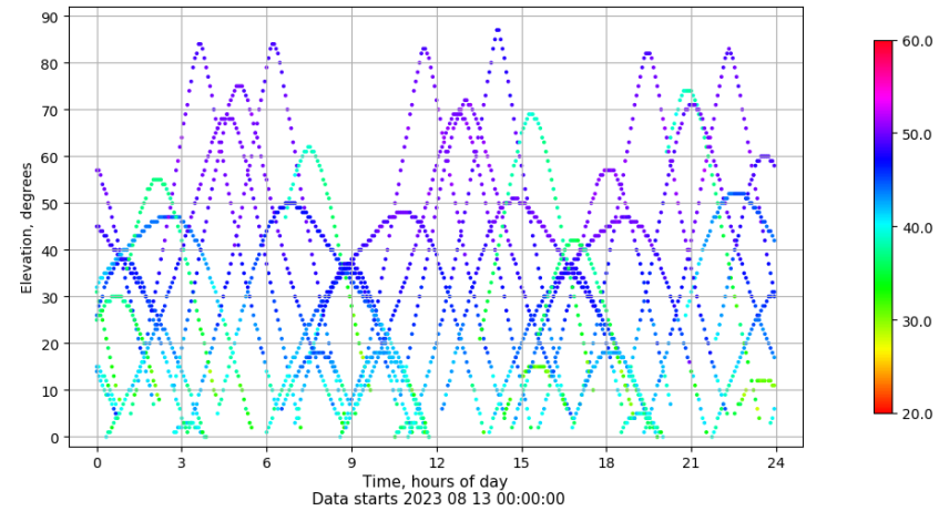
Time-elevation plot for station LP01. Signal to Noise S1C Data file LP0100ESP_R_2023225.xtr
