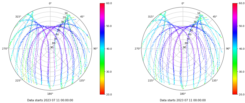
Skyplot for station LP01. Signal to Noise S1C Data file LP0100ESP_R_2023192.xtr Skyplot for station LP01. Signal to Noise S2C Data file LP0100ESP_R_2023192.xtr
