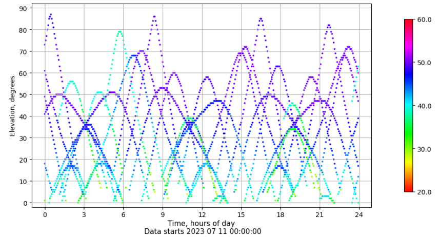
Time-elevation plot for station LP01. Signal to Noise S1C Data file LP0100ESP_R_2023192.xtr
