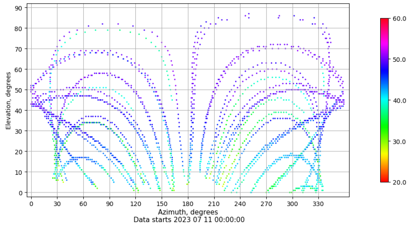
Azimuth-elevation plot for station LP01. Signal to Noise S1C Data file LP0100ESP_R_2023192.xtr
