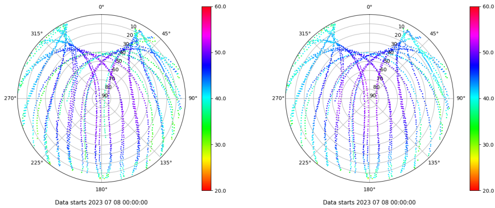
Skyplot for station LP01. Signal to Noise S1C Data file LP0100ESP_R_2023189.xtr Skyplot for station LP01. Signal to Noise S2C Data file LP0100ESP_R_2023189.xtr
