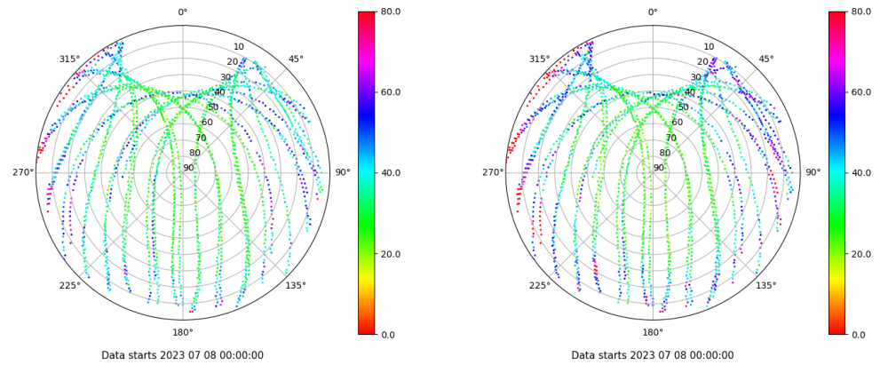
Skyplot for station LP01. Parameter M1C Data file LP0100ESP_R_2023189.xtr Skyplot for station LP01. Parameter M2C Data file LP0100ESP_R_2023189.xtr
