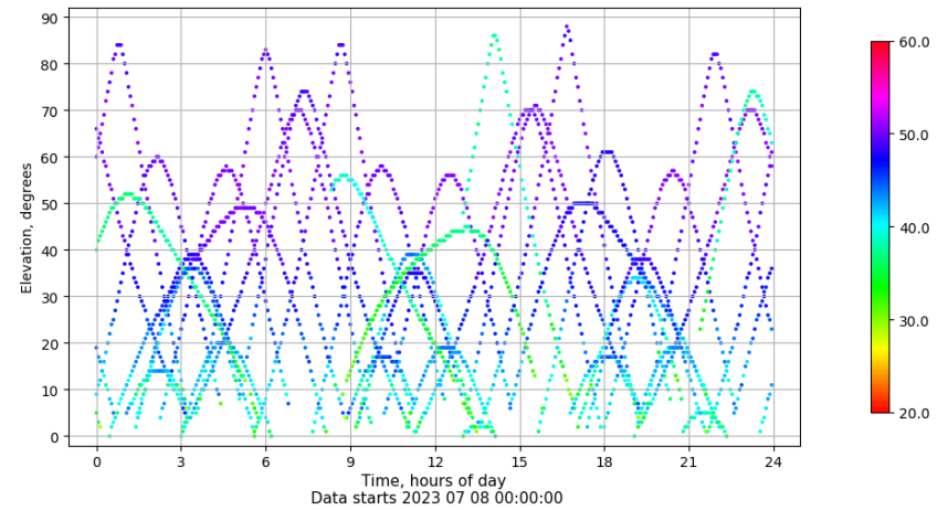
Time-elevation plot for station LP01. Signal to Noise S1C Data file LP0100ESP_R_2023189.xtr
