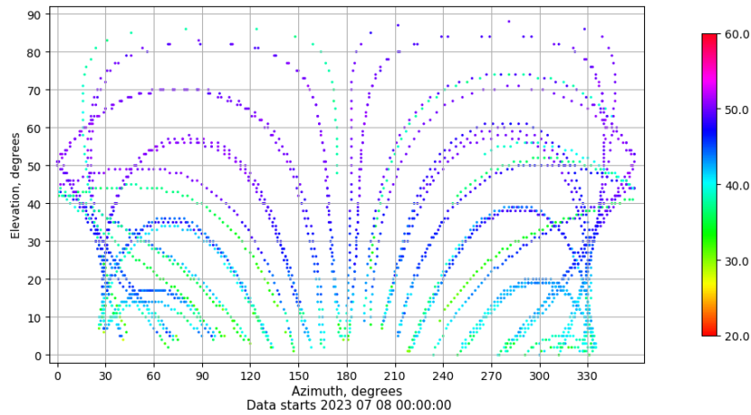
Azimuth-elevation plot for station LP01. Signal to Noise S1C Data file LP0100ESP_R_2023189.xtr
