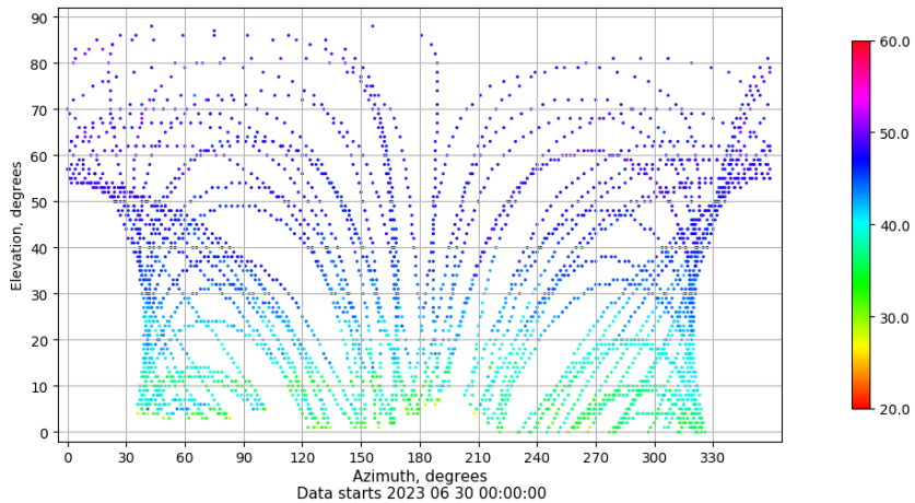
Azimuth-elevation plot for station LP01. Signal to Noise S1C Data file LP0100ESP_R_2023181.xtr
