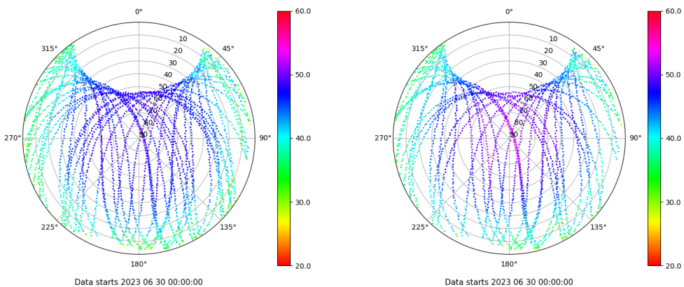
Skyplot for station LP01. Signal to Noise S1C Data file LP0100ESP_R_2023181.xtr Skyplot for station LP01. Signal to Noise S2X Data file LP0100ESP_R_2023181.xtr
