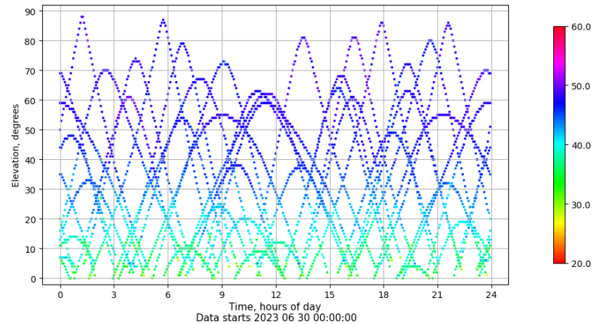
Time-elevation plot for station LP01. Signal to Noise S1C Data file LP0100ESP_R_2023181.xtr
