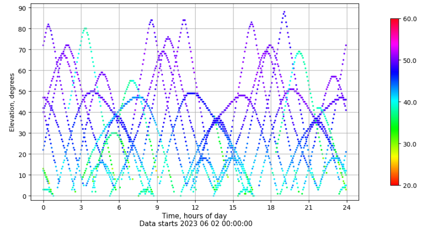
Time-elevation plot for station LP01. Signal to Noise S1C Data file LP0100ESP_R_2023153.xtr
