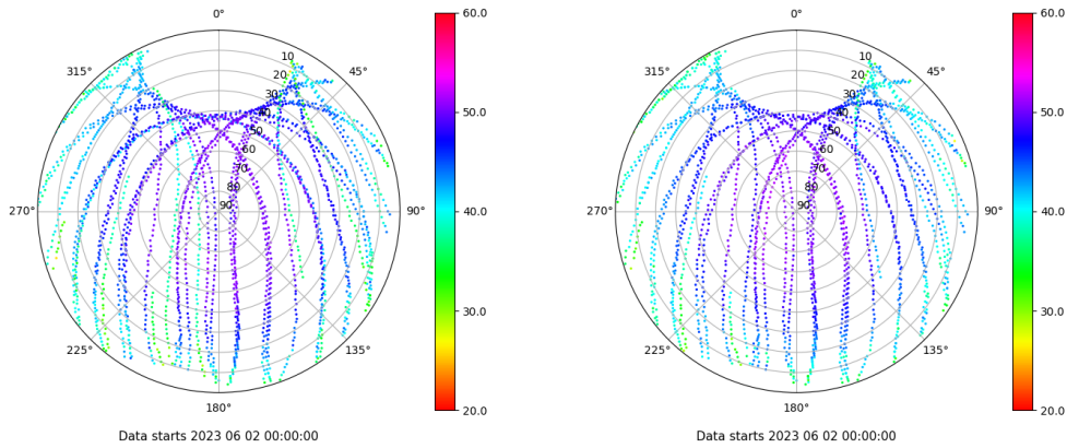
Skyplot for station LP01. Signal to Noise S1C Data file LP0100ESP_R_2023153.xtr Skyplot for station LP01. Signal to Noise S2C Data file LP0100ESP_R_2023153.xtr
