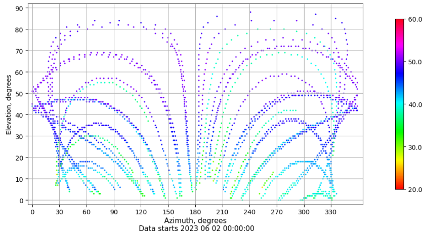
Azimuth-elevation plot for station LP01. Signal to Noise S1C Data file LP0100ESP_R_2023153.xtr
