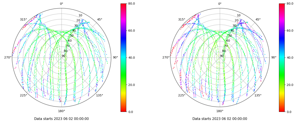
Skyplot for station LP01. Parameter M1C Data file LP0100ESP_R_2023153.xtr Skyplot for station LP01. Parameter M2C Data file LP0100ESP_R_2023153.xtr
