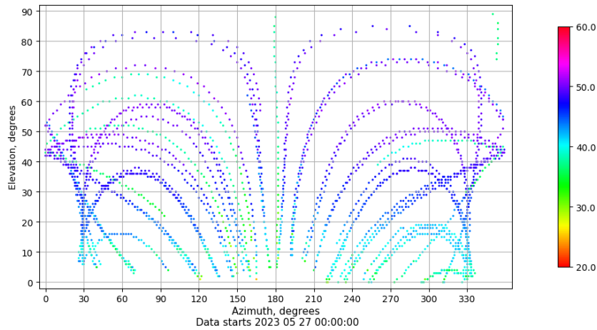
Azimuth-elevation plot for station LP01. Signal to Noise S1C Data file LP0100ESP_R_2023147.xtr
