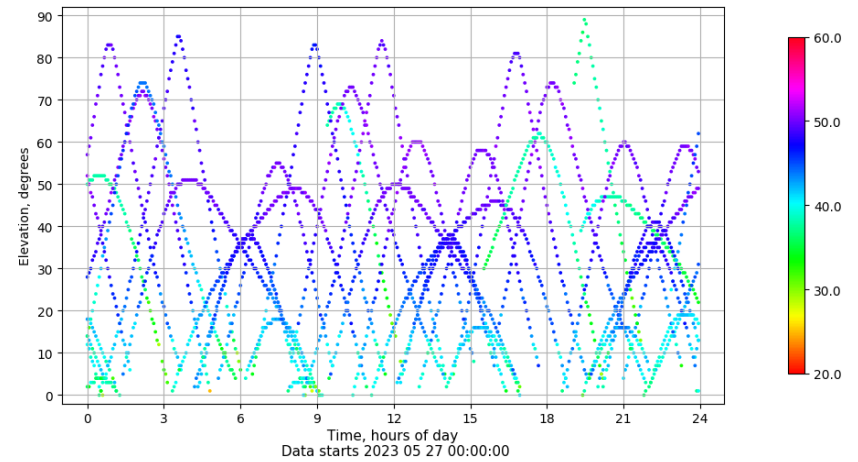
Time-elevation plot for station LP01. Signal to Noise S1C Data file LP0100ESP_R_2023147.xtr
