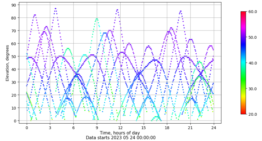
Time-elevation plot for station LP01. Signal to Noise S1C Data file LP0100ESP_R_2023144.xtr
