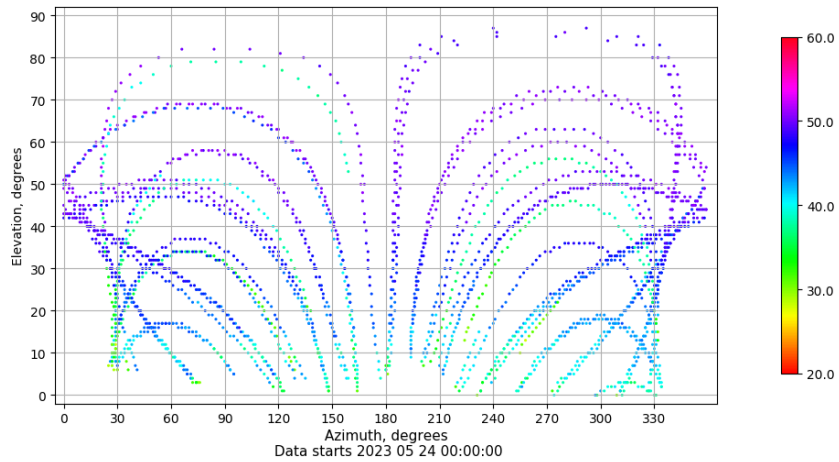
Azimuth-elevation plot for station LP01. Signal to Noise S1C Data file LP0100ESP_R_2023144.xtr
