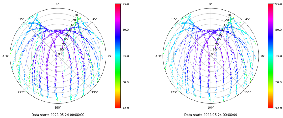
Skyplot for station LP01. Signal to Noise S1C Data file LP0100ESP_R_2023144.xtr Skyplot for station LP01. Signal to Noise S2C Data file LP0100ESP_R_2023144.xtr
