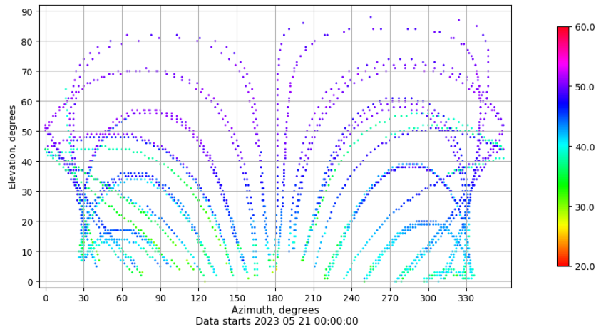
Azimuth-elevation plot for station LP01. Signal to Noise S1C Data file LP0100ESP_R_2023141.xtr
