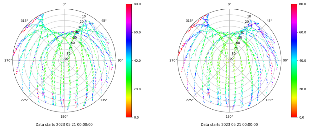
Skyplot for station LP01. Parameter M1C Data file LP0100ESP_R_2023141.xtr Skyplot for station LP01. Parameter M2C Data file LP0100ESP_R_2023141.xtr
