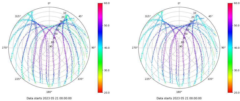
Skyplot for station LP01. Signal to Noise S1C Data file LP0100ESP_R_2023141.xtr Skyplot for station LP01. Signal to Noise S2C Data file LP0100ESP_R_2023141.xtr
