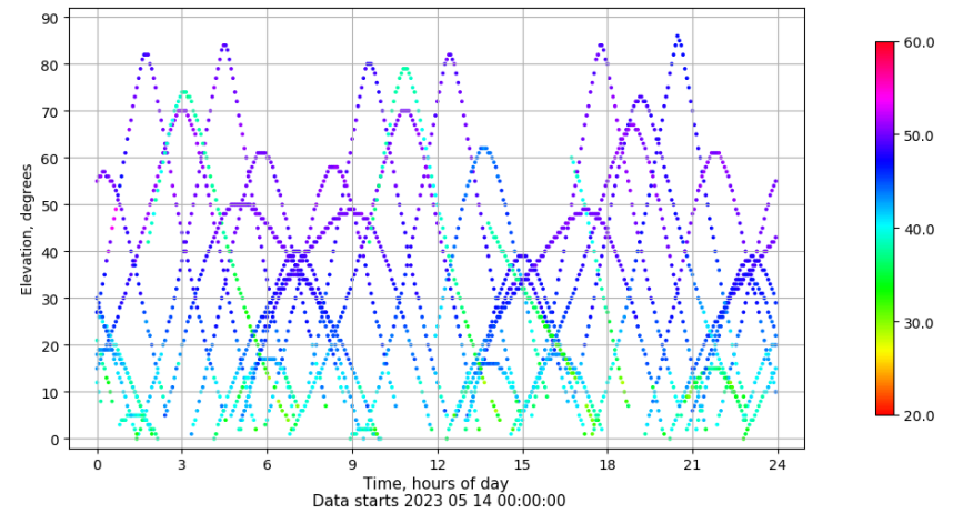
Time-elevation plot for station LP01. Signal to Noise S1C Data file LP0100ESP_R_2023134.xtr
