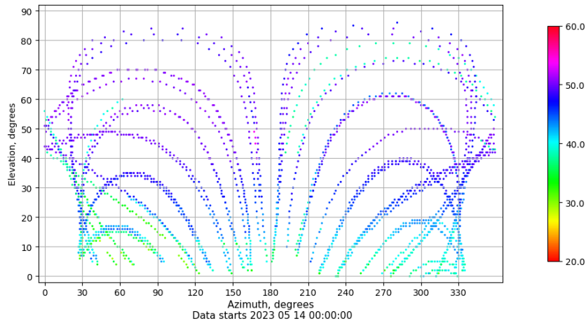
Azimuth-elevation plot for station LP01. Signal to Noise S1C Data file LP0100ESP_R_2023134.xtr
