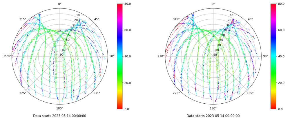
Skyplot for station LP01. Parameter M1C Data file LP0100ESP_R_2023134.xtr Skyplot for station LP01. Parameter M2C Data file LP0100ESP_R_2023134.xtr
