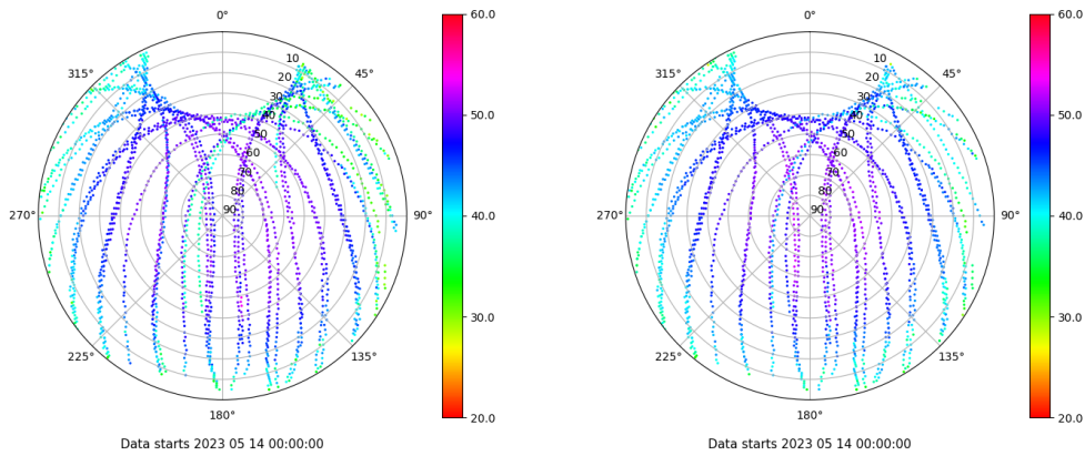
Skyplot for station LP01. Signal to Noise S1C Data file LP0100ESP_R_2023134.xtr Skyplot for station LP01. Signal to Noise S2C Data file LP0100ESP_R_2023134.xtr
