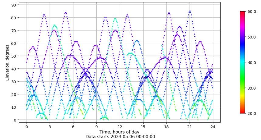
Time-elevation plot for station LP01. Signal to Noise S1C Data file LP0100ESP_R_2023126.xtr
