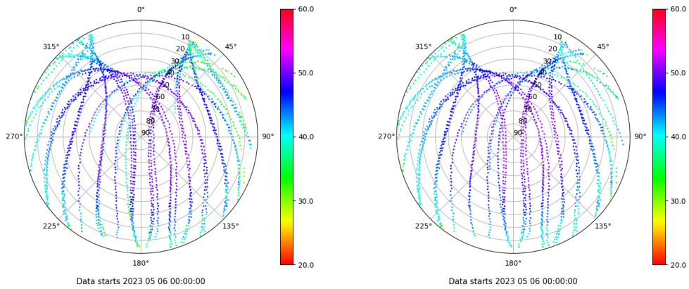
Skyplot for station LP01. Signal to Noise S1C Data file LP0100ESP_R_2023126.xtr Skyplot for station LP01. Signal to Noise S2C Data file LP0100ESP_R_2023126.xtr
