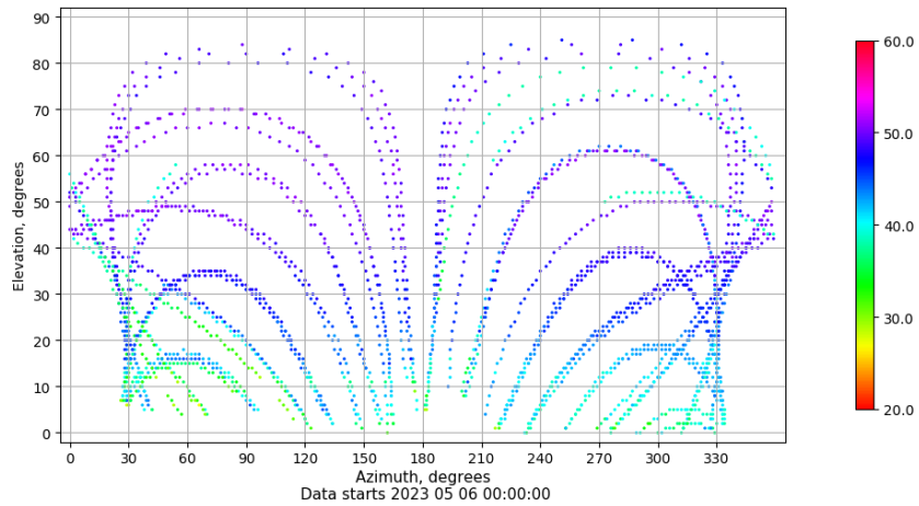
Azimuth-elevation plot for station LP01. Signal to Noise S1C Data file LP0100ESP_R_2023126.xtr
