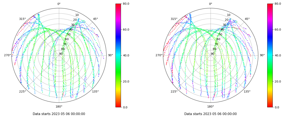
Skyplot for station LP01. Parameter M1C Data file LP0100ESP_R_2023126.xtr Skyplot for station LP01. Parameter M2C Data file LP0100ESP_R_2023126.xtr
