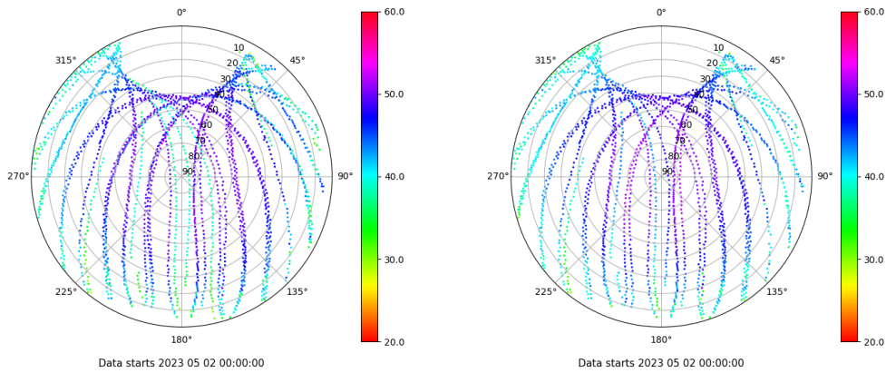
Skyplot for station LP01. Signal to Noise S1C Data file LP0100ESP_R_2023122.xtr Skyplot for station LP01. Signal to Noise S2C Data file LP0100ESP_R_2023122.xtr
