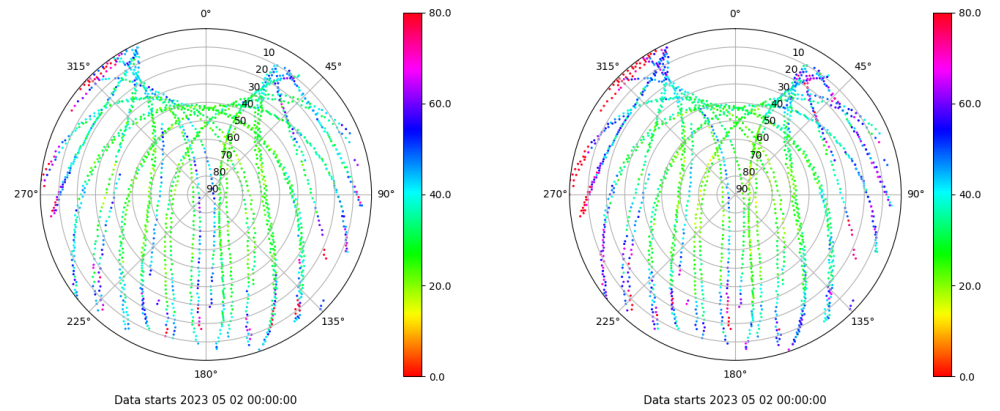
Skyplot for station LP01. Parameter M1C Data file LP0100ESP_R_2023122.xtr Skyplot for station LP01. Parameter M2C Data file LP0100ESP_R_2023122.xtr
