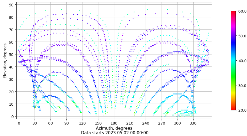
Azimuth-elevation plot for station LP01. Signal to Noise S1C Data file LP0100ESP_R_2023122.xtr
