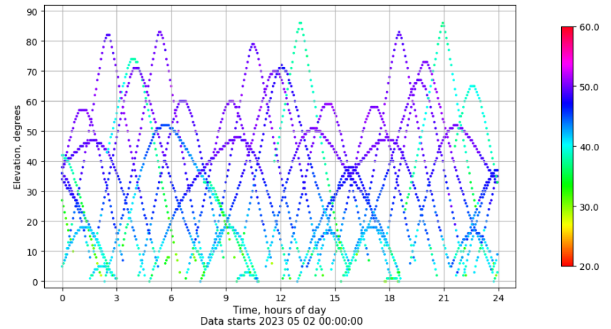
Time-elevation plot for station LP01. Signal to Noise S1C Data file LP0100ESP_R_2023122.xtr
