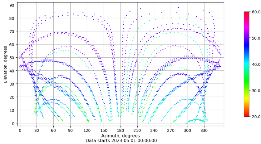
Azimuth-elevation plot for station LP01. Signal to Noise S1C Data file LP0100ESP_R_2023121.xtr
