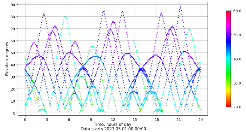
Time-elevation plot for station LP01. Signal to Noise S1C Data file LP0100ESP_R_2023121.xtr
