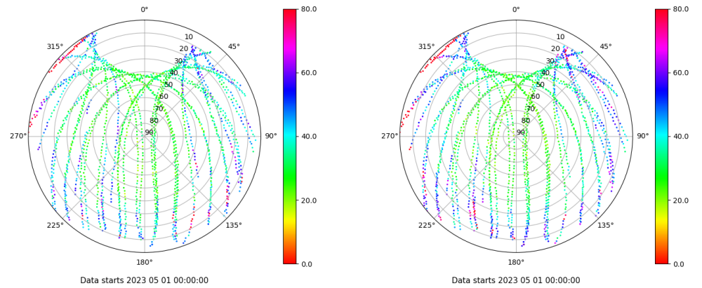
Skyplot for station LP01. Parameter M1C Data file LP0100ESP_R_2023121.xtr Skyplot for station LP01. Parameter M2C Data file LP0100ESP_R_2023121.xtr
