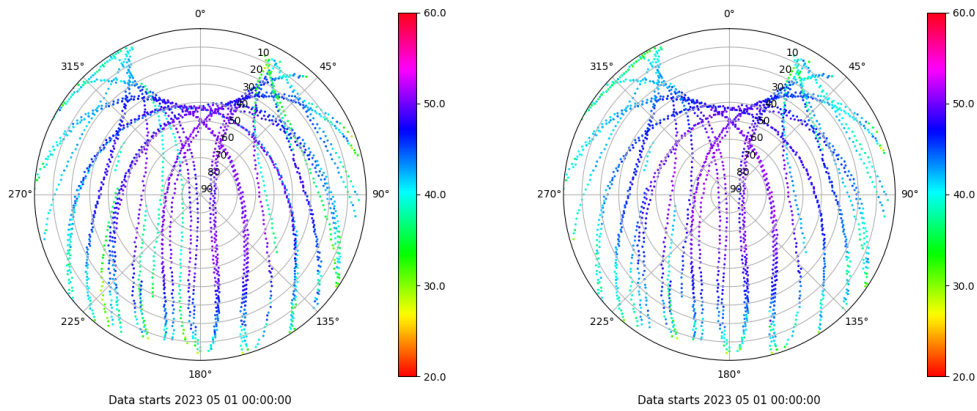
Skyplot for station LP01. Signal to Noise S1C Data file LP0100ESP_R_2023121.xtr Skyplot for station LP01. Signal to Noise S2C Data file LP0100ESP_R_2023121.xtr
