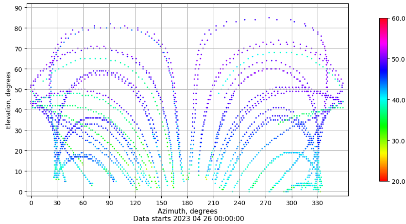
Azimuth-elevation plot for station LP01. Signal to Noise S1C Data file LP0100ESP_R_2023116.xtr
