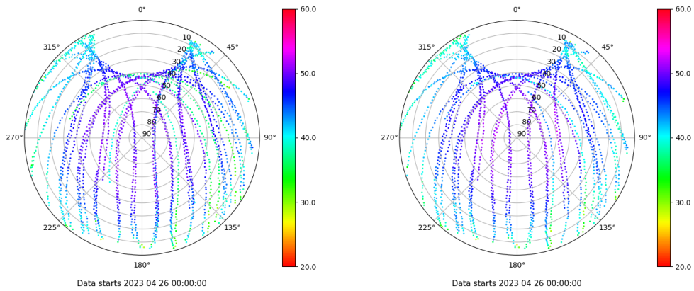
Skyplot for station LP01. Signal to Noise S1C Data file LP0100ESP_R_2023116.xtr Skyplot for station LP01. Signal to Noise S2C Data file LP0100ESP_R_2023116.xtr
