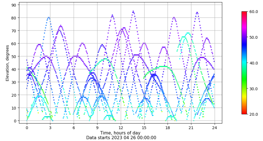
Time-elevation plot for station LP01. Signal to Noise S1C Data file LP0100ESP_R_2023116.xtr
