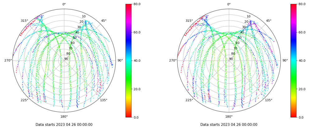
Skyplot for station LP01. Parameter M1C Data file LP0100ESP_R_2023116.xtr Skyplot for station LP01. Parameter M2C Data file LP0100ESP_R_2023116.xtr
