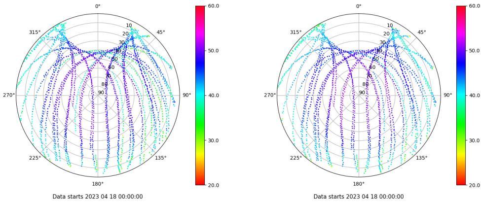
Skyplot for station LP01. Signal to Noise S1C Data file LP0100ESP_R_2023108.xtr Skyplot for station LP01. Signal to Noise S2C Data file LP0100ESP_R_2023108.xtr
