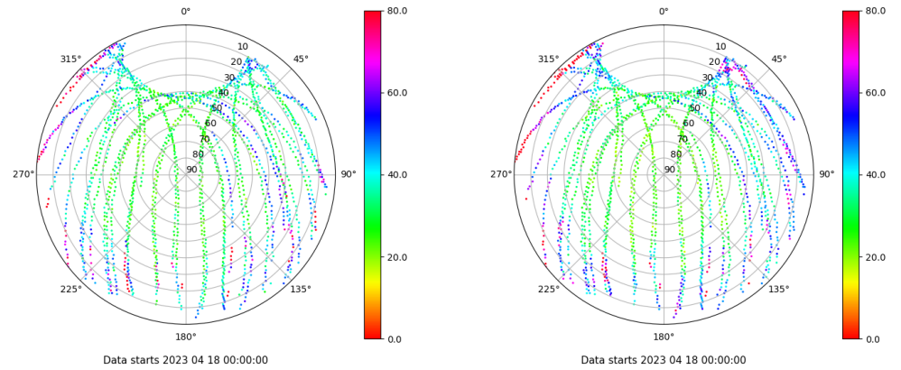
Skyplot for station LP01. Parameter M1C Data file LP0100ESP_R_2023108.xtr Skyplot for station LP01. Parameter M2C Data file LP0100ESP_R_2023108.xtr
