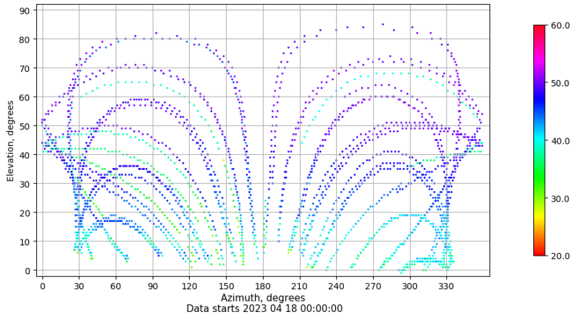
Azimuth-elevation plot for station LP01. Signal to Noise S1C Data file LP0100ESP_R_2023108.xtr
