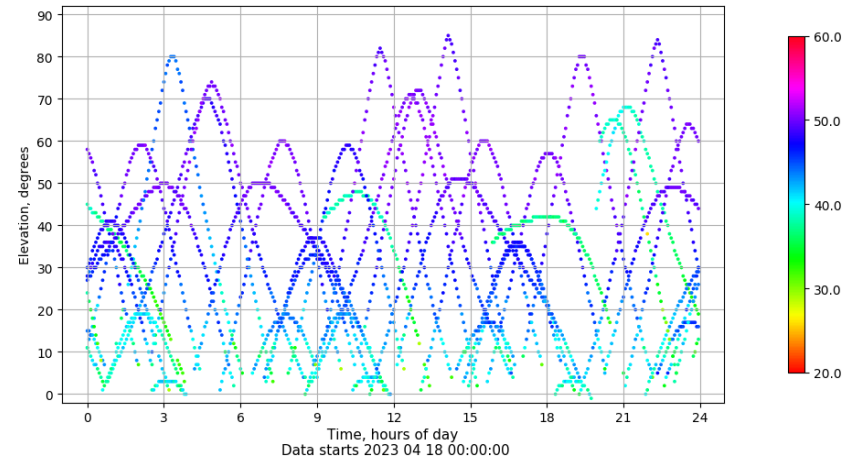
Time-elevation plot for station LP01. Signal to Noise S1C Data file LP0100ESP_R_2023108.xtr
