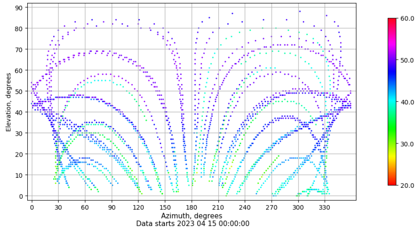
Azimuth-elevation plot for station LP01. Signal to Noise S1C Data file LP0100ESP_R_2023105.xtr
