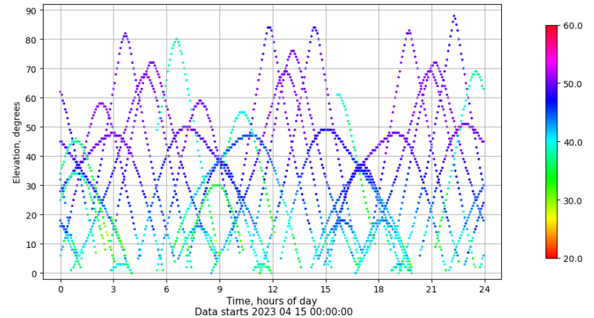
Time-elevation plot for station LP01. Signal to Noise S1C Data file LP0100ESP_R_2023105.xtr
