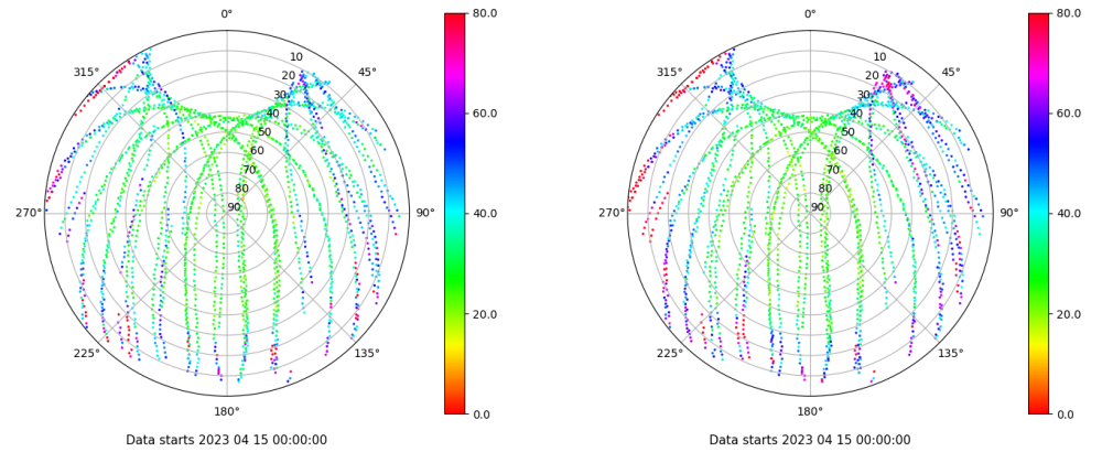
Skyplot for station LP01. Parameter M1C Data file LP0100ESP_R_2023105.xtr Skyplot for station LP01. Parameter M2C Data file LP0100ESP_R_2023105.xtr
