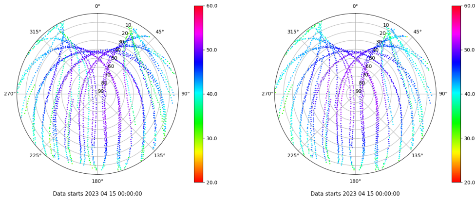
Skyplot for station LP01. Signal to Noise S1C Data file LP0100ESP_R_2023105.xtr Skyplot for station LP01. Signal to Noise S2C Data file LP0100ESP_R_2023105.xtr
