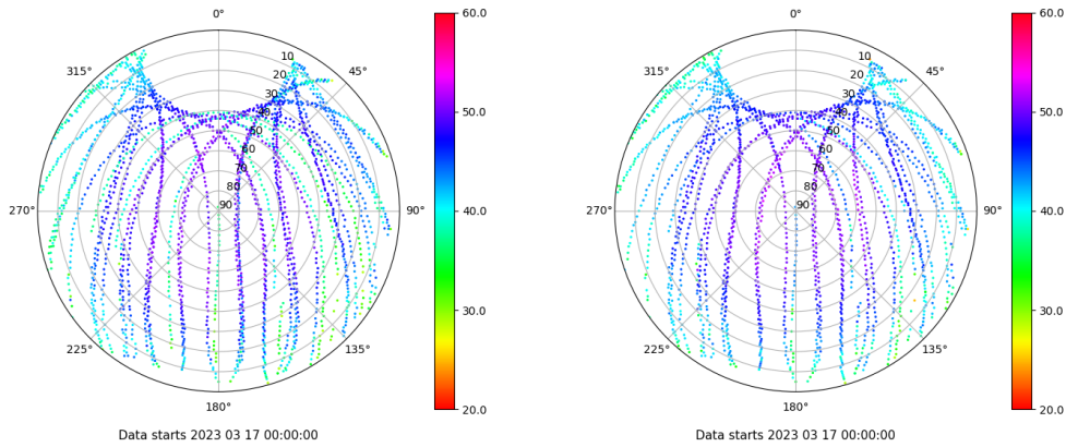
Skyplot for station LP01. Signal to Noise S1C Data file LP0100ESP_R_2023076.xtr Skyplot for station LP01. Signal to Noise S2C Data file LP0100ESP_R_2023076.xtr
