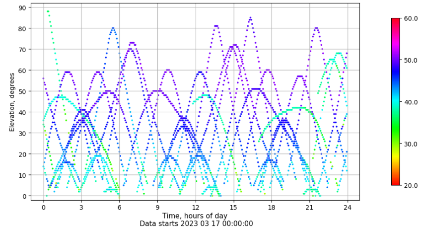
Time-elevation plot for station LP01. Signal to Noise S1C Data file LP0100ESP_R_2023076.xtr
