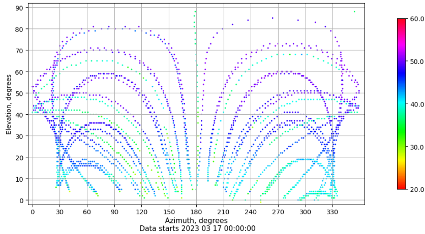
Azimuth-elevation plot for station LP01. Signal to Noise S1C Data file LP0100ESP_R_2023076.xtr
