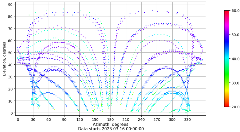
Azimuth-elevation plot for station LP01. Signal to Noise S1C Data file LP0100ESP_R_2023075.xtr
