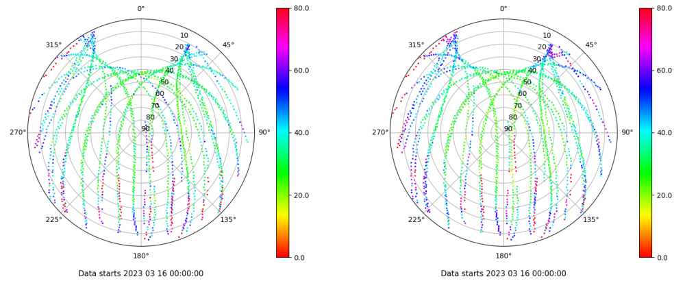
Skyplot for station LP01. Parameter M1C Data file LP0100ESP_R_2023075.xtr Skyplot for station LP01. Parameter M2C Data file LP0100ESP_R_2023075.xtr
