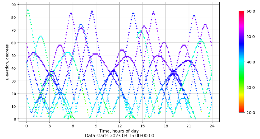
Time-elevation plot for station LP01. Signal to Noise S1C Data file LP0100ESP_R_2023075.xtr
