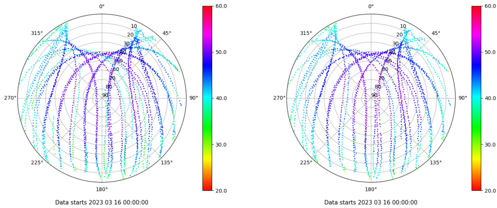
Skyplot for station LP01. Signal to Noise S1C Data file LP0100ESP_R_2023075.xtr Skyplot for station LP01. Signal to Noise S2C Data file LP0100ESP_R_2023075.xtr
