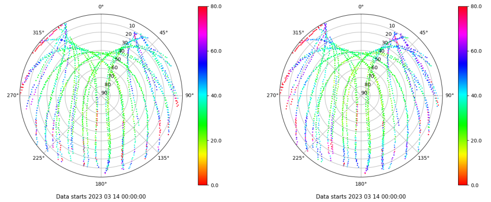
Skyplot for station LP01. Parameter M1C Data file LP0100ESP_R_2023073.xtr Skyplot for station LP01. Parameter M2C Data file LP0100ESP_R_2023073.xtr
