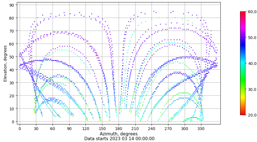
Azimuth-elevation plot for station LP01. Signal to Noise S1C Data file LP0100ESP_R_2023073.xtr
