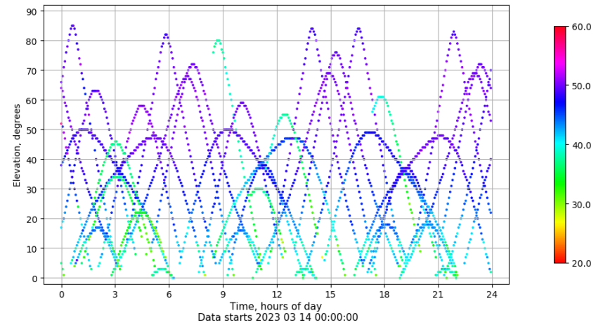
Time-elevation plot for station LP01. Signal to Noise S1C Data file LP0100ESP_R_2023073.xtr
