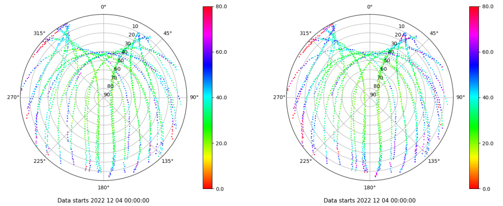
Skyplot for station LP01. Parameter M1C Data file LP0100ESP_R_2022338.xtr Skyplot for station LP01. Parameter M2C Data file LP0100ESP_R_2022338.xtr
