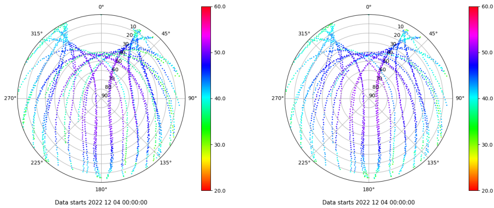
Skyplot for station LP01. Signal to Noise S1C Data file LP0100ESP_R_2022338.xtr Skyplot for station LP01. Signal to Noise S2C Data file LP0100ESP_R_2022338.xtr
