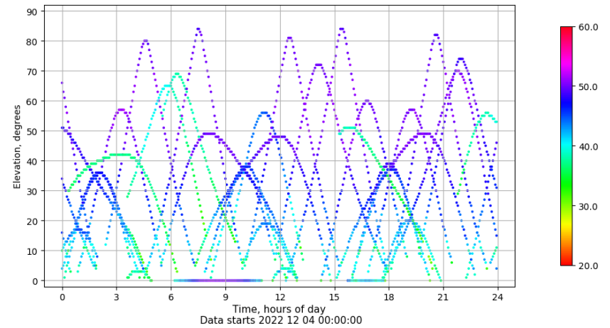
Time-elevation plot for station LP01. Signal to Noise S1C Data file LP0100ESP_R_2022338.xtr
