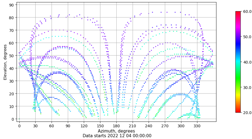
Azimuth-elevation plot for station LP01. Signal to Noise S1C Data file LP0100ESP_R_2022338.xtr
