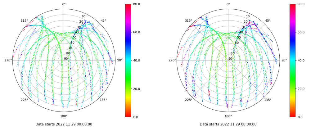
Skyplot for station LP01. Parameter M1C Data file LP0100ESP_R_2022333.xtr Skyplot for station LP01. Parameter M2C Data file LP0100ESP_R_2022333.xtr
