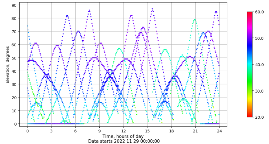
Time-elevation plot for station LP01. Signal to Noise S1C Data file LP0100ESP_R_2022333.xtr
