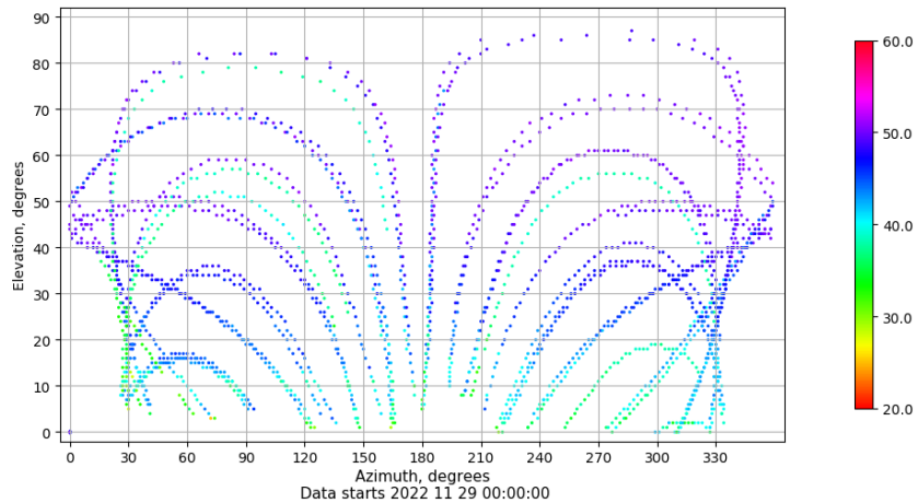
Azimuth-elevation plot for station LP01. Signal to Noise S1C Data file LP0100ESP_R_2022333.xtr
