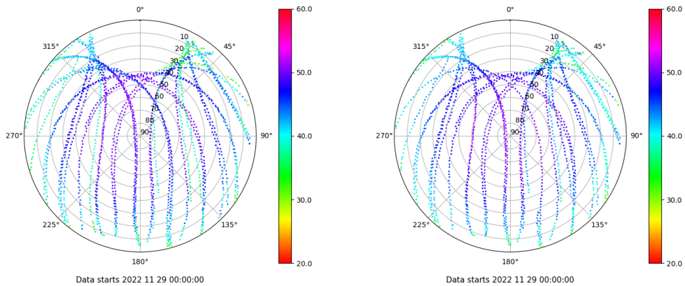
Skyplot for station LP01. Signal to Noise S1C Data file LP0100ESP_R_2022333.xtr Skyplot for station LP01. Signal to Noise S2C Data file LP0100ESP_R_2022333.xtr
