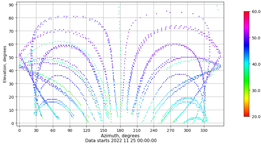
Azimuth-elevation plot for station LP01. Signal to Noise S1C Data file LP0100ESP_R_2022329.xtr
