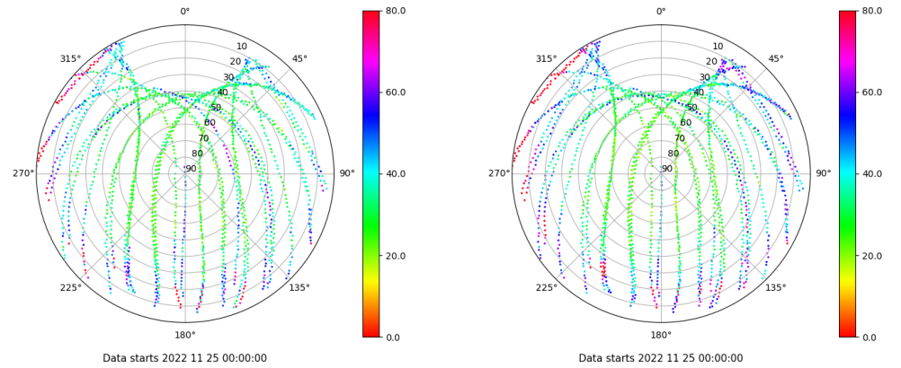
Skyplot for station LP01. Parameter M1C Data file LP0100ESP_R_2022329.xtr Skyplot for station LP01. Parameter M2C Data file LP0100ESP_R_2022329.xtr
