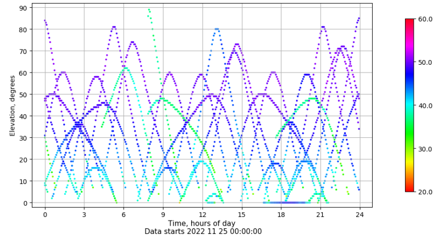
Time-elevation plot for station LP01. Signal to Noise S1C Data file LP0100ESP_R_2022329.xtr
