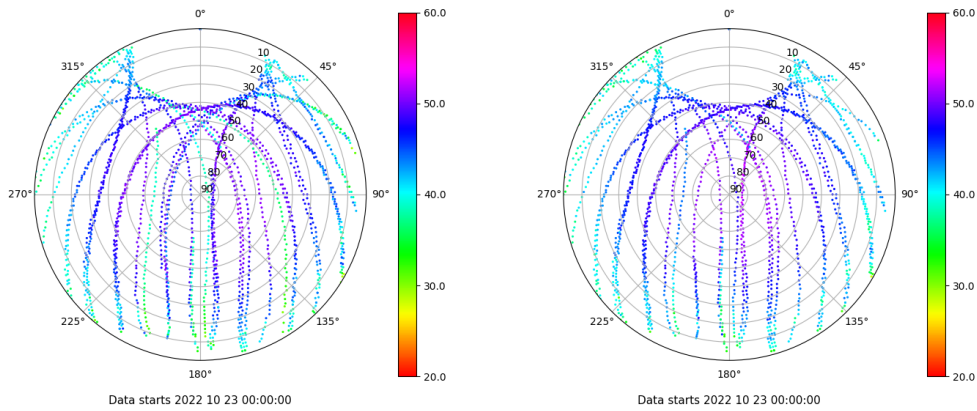
Skyplot for station LP01. Signal to Noise S1C Data file LP0100ESP_R_2022296.xtr Skyplot for station LP01. Signal to Noise S2C Data file LP0100ESP_R_2022296.xtr
