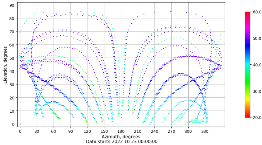
Azimuth-elevation plot for station LP01. Signal to Noise S1C Data file LP0100ESP_R_2022296.xtr
