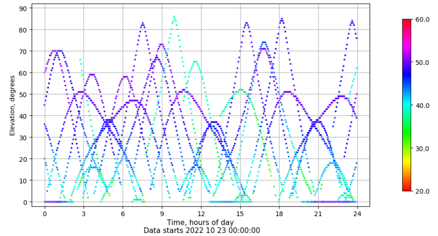
Time-elevation plot for station LP01. Signal to Noise S1C Data file LP0100ESP_R_2022296.xtr
