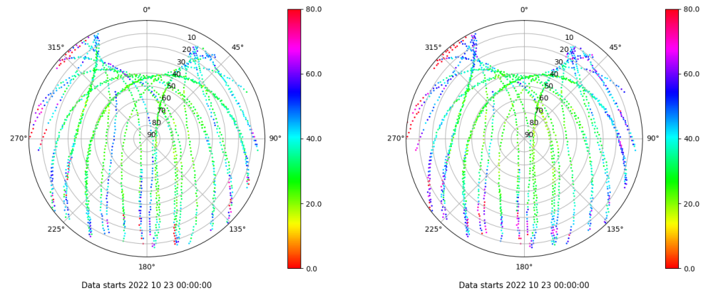
Skyplot for station LP01. Parameter M1C Data file LP0100ESP_R_2022296.xtr Skyplot for station LP01. Parameter M2C Data file LP0100ESP_R_2022296.xtr
