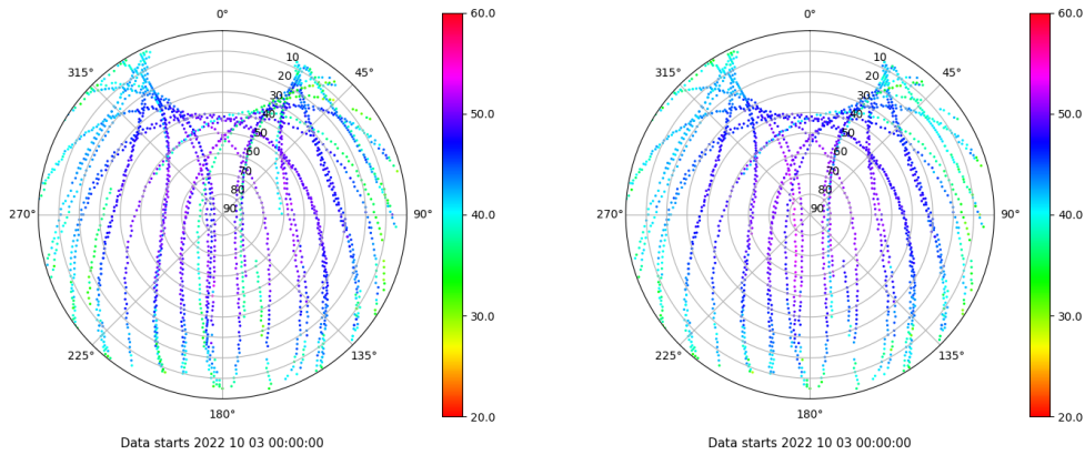
Skyplot for station LP01. Signal to Noise S1C Data file LP0100ESP_R_2022276.xtr Skyplot for station LP01. Signal to Noise S2C Data file LP0100ESP_R_2022276.xtr
