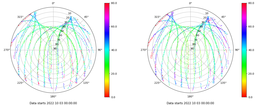
Skyplot for station LP01. Parameter M1C Data file LP0100ESP_R_2022276.xtr Skyplot for station LP01. Parameter M2C Data file LP0100ESP_R_2022276.xtr
