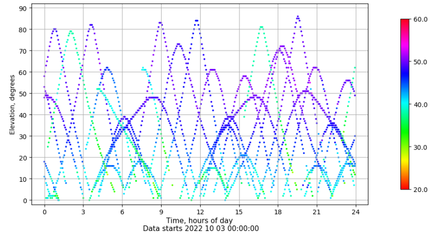
Time-elevation plot for station LP01. Signal to Noise S1C Data file LP0100ESP_R_2022276.xtr
