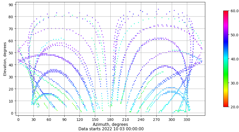
Azimuth-elevation plot for station LP01. Signal to Noise S1C Data file LP0100ESP_R_2022276.xtr
