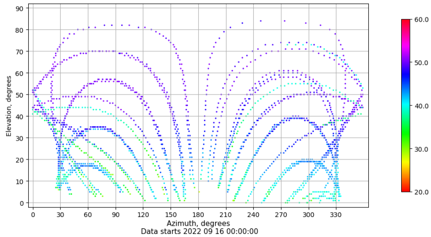
Azimuth-elevation plot for station LP01. Signal to Noise S1C Data file LP0100ESP_R_2022259.xtr
