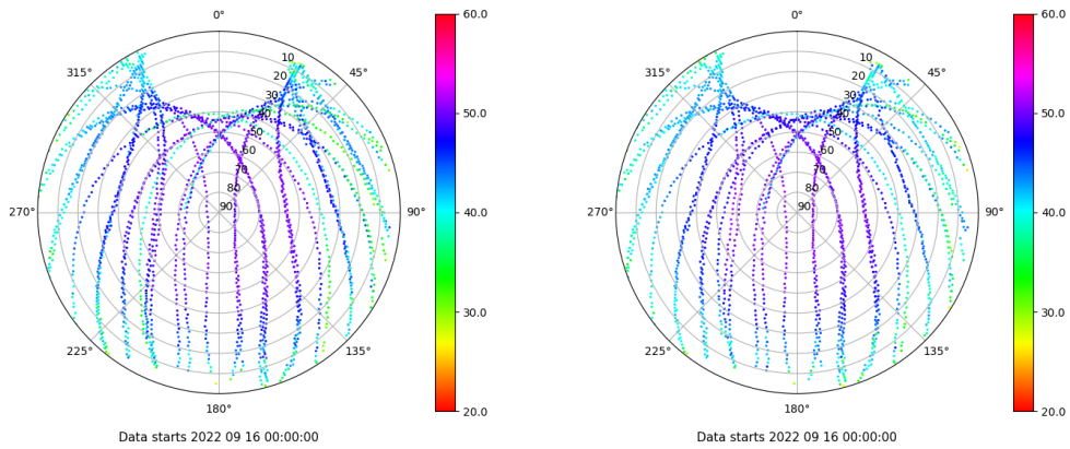
Skyplot for station LP01. Signal to Noise S1C Data file LP0100ESP_R_2022259.xtr Skyplot for station LP01. Signal to Noise S2C Data file LP0100ESP_R_2022259.xtr
