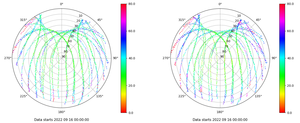
Skyplot for station LP01. Parameter M1C Data file LP0100ESP_R_2022259.xtr Skyplot for station LP01. Parameter M2C Data file LP0100ESP_R_2022259.xtr
