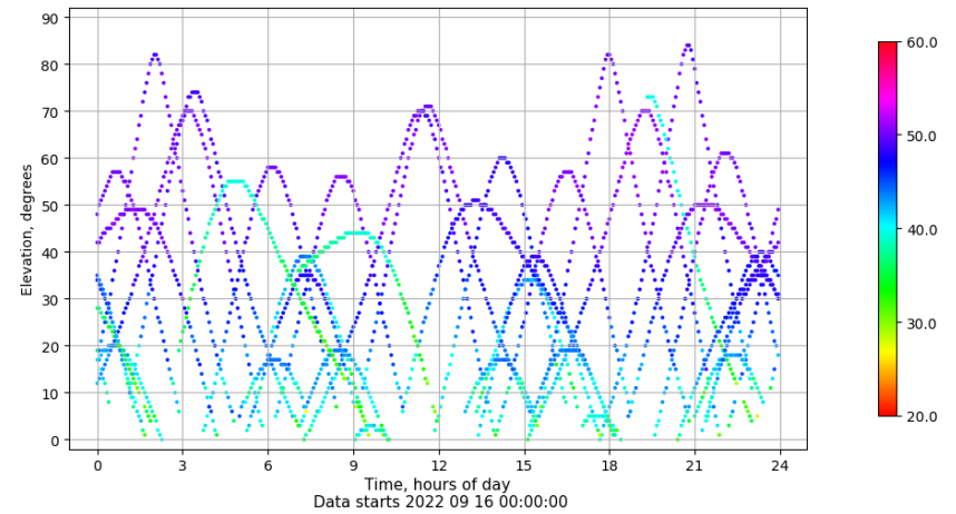
Time-elevation plot for station LP01. Signal to Noise S1C Data file LP0100ESP_R_2022259.xtr
