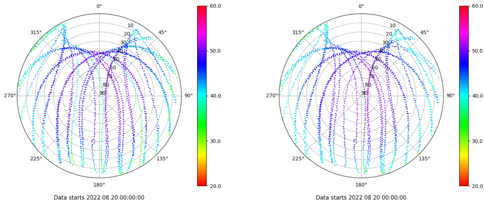
Skyplot for station LP01. Signal to Noise S1C Data file LP0100ESP_R_2022232.xtr Skyplot for station LP01. Signal to Noise S2C Data file LP0100ESP_R_2022232.xtr
