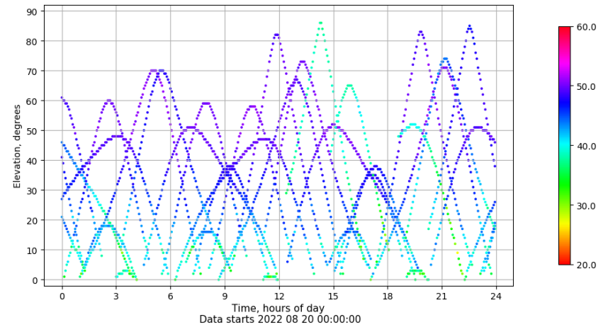
Time-elevation plot for station LP01. Signal to Noise S1C Data file LP0100ESP_R_2022232.xtr
