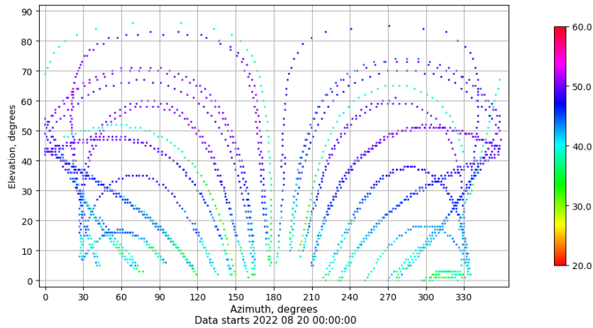
Azimuth-elevation plot for station LP01. Signal to Noise S1C Data file LP0100ESP_R_2022232.xtr
