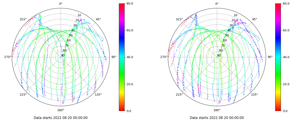
Skyplot for station LP01. Parameter M1C Data file LP0100ESP_R_2022232.xtr Skyplot for station LP01. Parameter M2C Data file LP0100ESP_R_2022232.xtr
