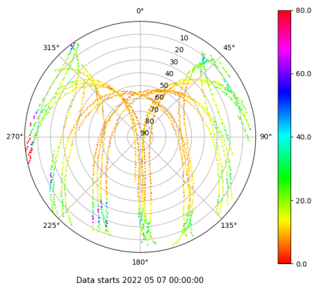
Skyplot for station LP01. Parameter M1X Data file LP0100ESP_R_2022127.xtr
