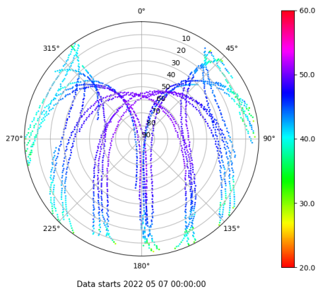
Skyplot for station LP01. Signal to Noise S1X Data file LP0100ESP_R_2022127.xtr
