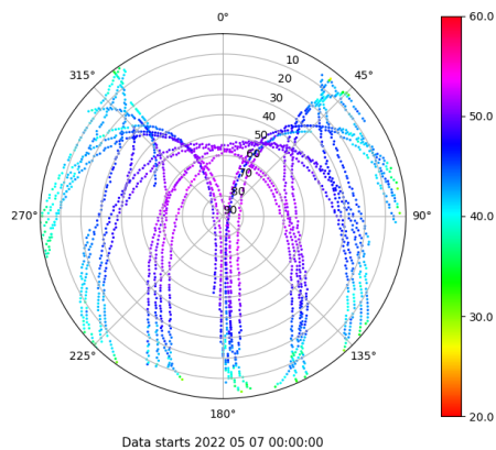
Skyplot for station LP01. Signal to Noise S5X Data file LP0100ESP_R_2022127.xtr
