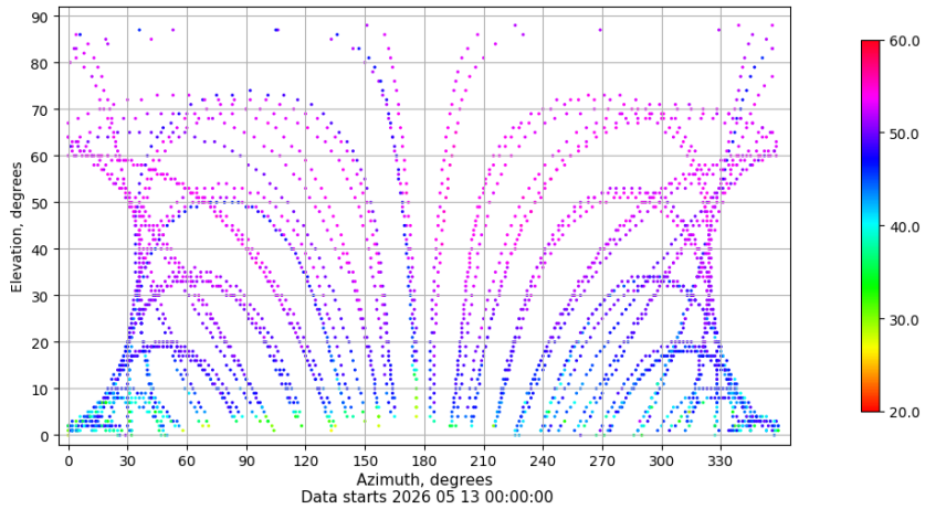
Azimuth-elevation plot for station LEON. Signal to Noise S1C Data file LEON00ESP_R_2026133.xtr
