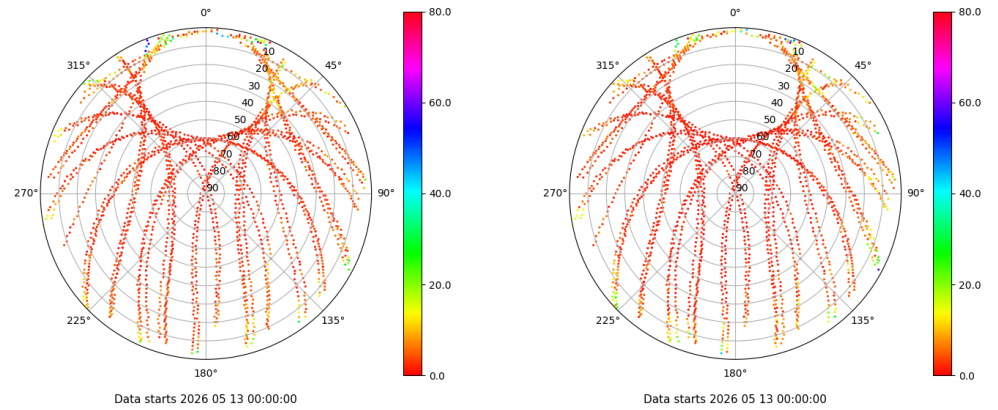
Skyplot for station LEON. Parameter M1C Data file LEON00ESP_R_2026133.xtr Skyplot for station LEON. Parameter M2P Data file LEON00ESP_R_2026133.xtr
