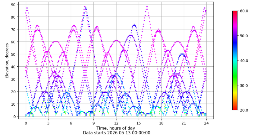
Time-elevation plot for station LEON. Signal to Noise S1C Data file LEON00ESP_R_2026133.xtr
