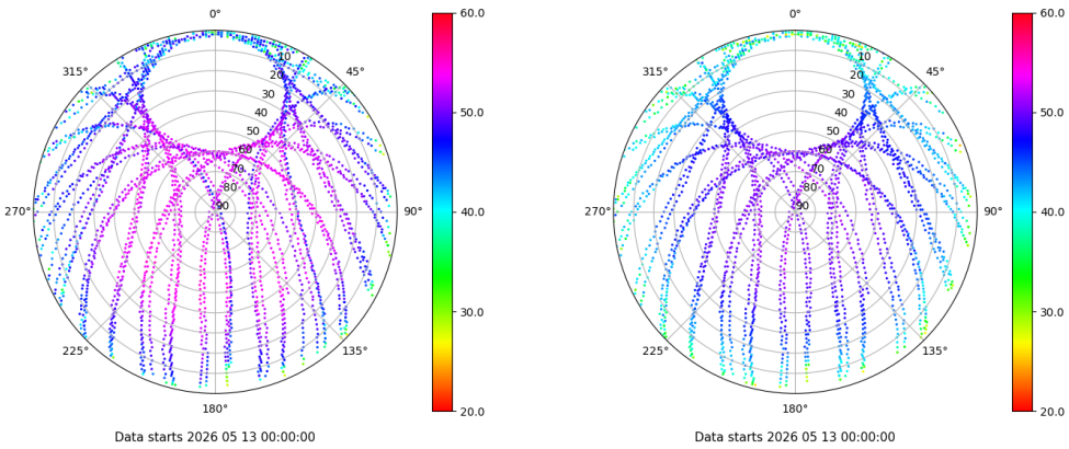
Skyplot for station LEON. Signal to Noise S1C Data file LEON00ESP_R_2026133.xtr Skyplot for station LEON. Signal to Noise S2P Data file LEON00ESP_R_2026133.xtr
