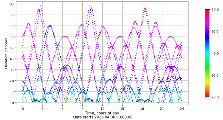
Time-elevation plot for station LEON. Signal to Noise S1C Data file LEON00ESP_R_2026096.xtr
