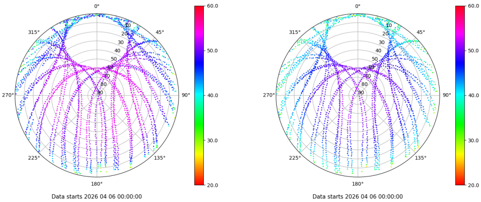
Skyplot for station LEON. Signal to Noise S1C Data file LEON00ESP_R_2026096.xtr Skyplot for station LEON. Signal to Noise S2P Data file LEON00ESP_R_2026096.xtr
