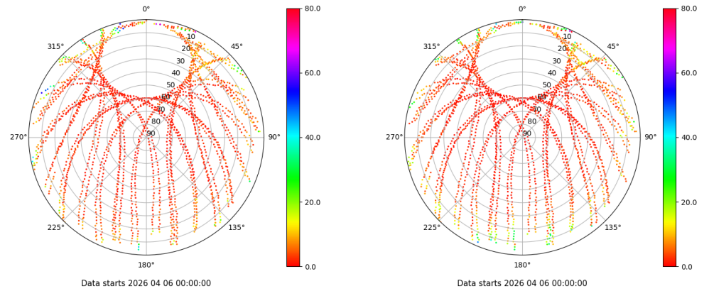
Skyplot for station LEON. Parameter M1C Data file LEON00ESP_R_2026096.xtr Skyplot for station LEON. Parameter M2P Data file LEON00ESP_R_2026096.xtr
