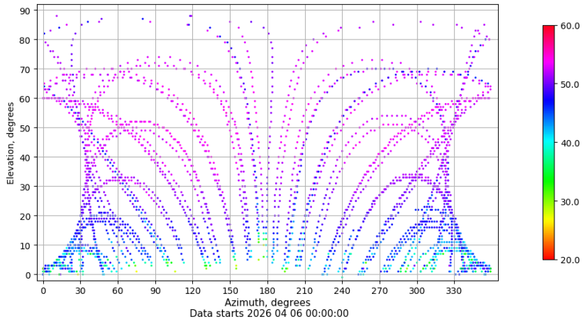
Azimuth-elevation plot for station LEON. Signal to Noise S1C Data file LEON00ESP_R_2026096.xtr
