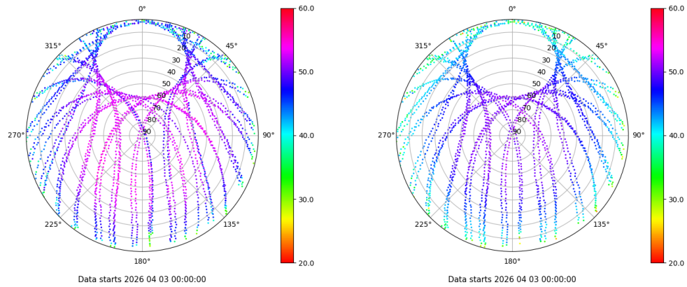
Skyplot for station LEON. Signal to Noise S1C Data file LEON00ESP_R_2026093.xtr Skyplot for station LEON. Signal to Noise S2P Data file LEON00ESP_R_2026093.xtr
