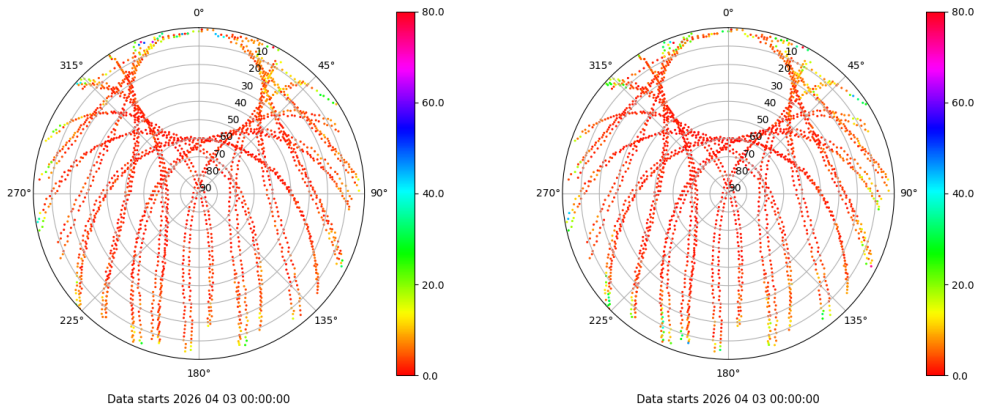
Skyplot for station LEON. Parameter M1C Data file LEON00ESP_R_2026093.xtr Skyplot for station LEON. Parameter M2P Data file LEON00ESP_R_2026093.xtr
