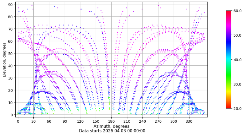
Azimuth-elevation plot for station LEON. Signal to Noise S1C Data file LEON00ESP_R_2026093.xtr
