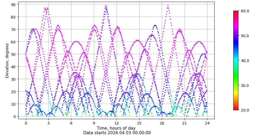
Time-elevation plot for station LEON. Signal to Noise S1C Data file LEON00ESP_R_2026093.xtr
