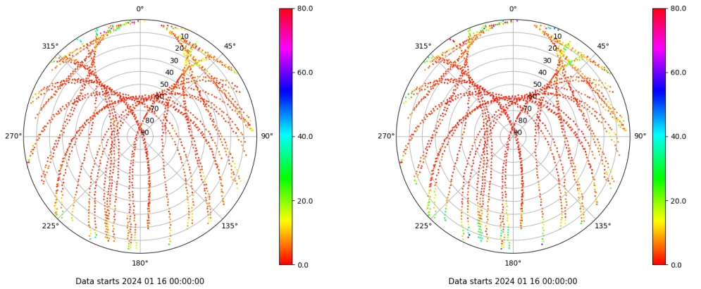
Skyplot for station LEON. Parameter M1C Data file LEON00ESP_R_2024016.xtr Skyplot for station LEON. Parameter M2P Data file LEON00ESP_R_2024016.xtr
