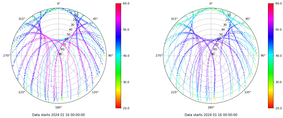
Skyplot for station LEON. Signal to Noise S1C Data file LEON00ESP_R_2024016.xtr Skyplot for station LEON. Signal to Noise S2P Data file LEON00ESP_R_2024016.xtr
