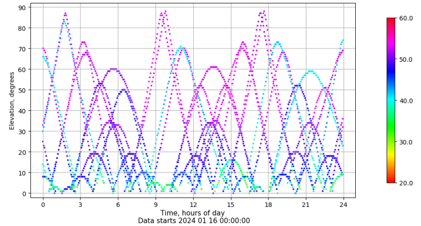
Time-elevation plot for station LEON. Signal to Noise S1C Data file LEON00ESP_R_2024016.xtr
