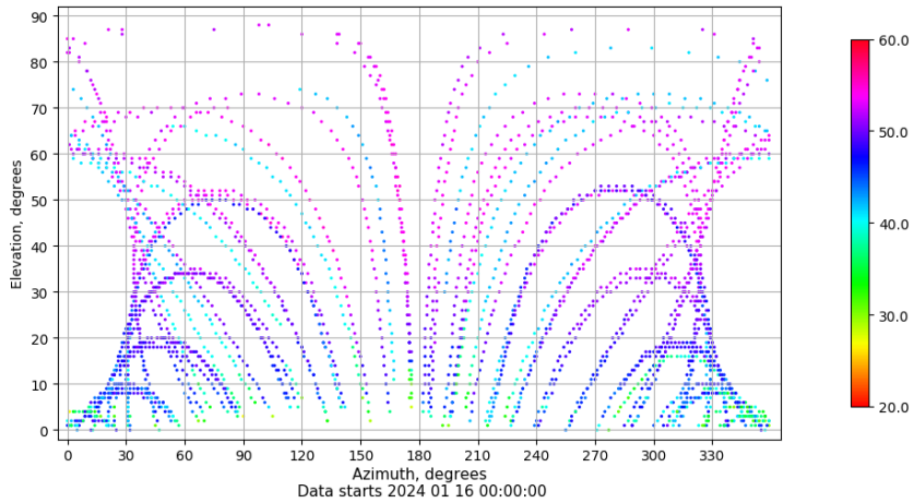
Azimuth-elevation plot for station LEON. Signal to Noise S1C Data file LEON00ESP_R_2024016.xtr
