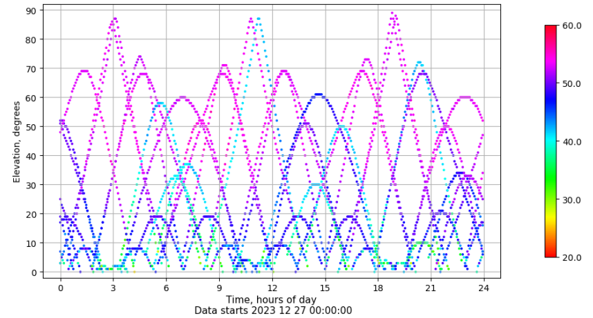
Time-elevation plot for station LEON. Signal to Noise S1C Data file LEON00ESP_R_2023361.xtr
