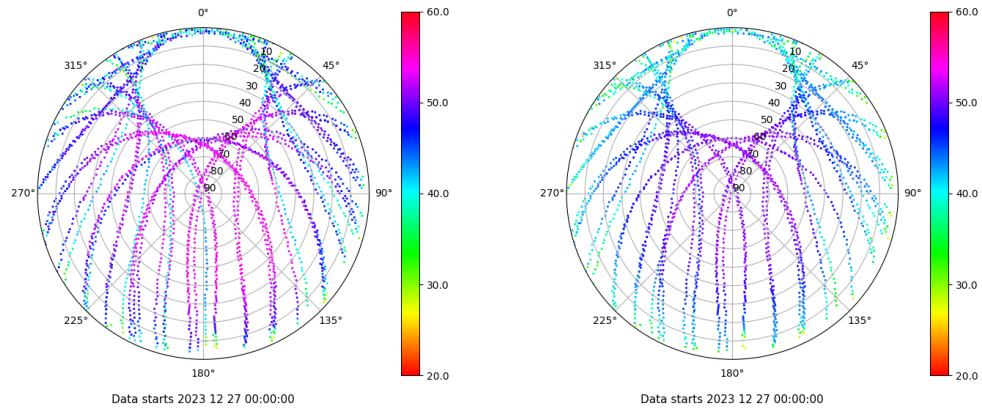
Skyplot for station LEON. Signal to Noise S1C Data file LEON00ESP_R_2023361.xtr Skyplot for station LEON. Signal to Noise S2P Data file LEON00ESP_R_2023361.xtr
