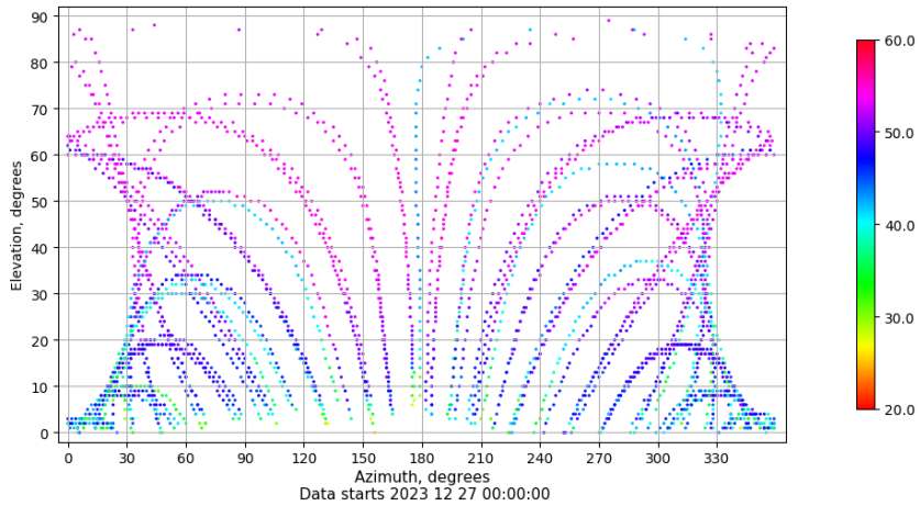
Azimuth-elevation plot for station LEON. Signal to Noise S1C Data file LEON00ESP_R_2023361.xtr
