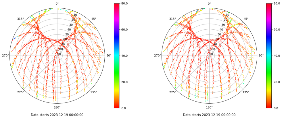
Skyplot for station LEON. Parameter M1C Data file LEON00ESP_R_2023353.xtr Skyplot for station LEON. Parameter M2P Data file LEON00ESP_R_2023353.xtr
