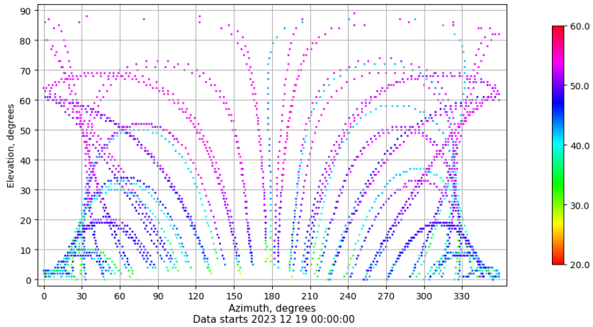
Azimuth-elevation plot for station LEON. Signal to Noise S1C Data file LEON00ESP_R_2023353.xtr
