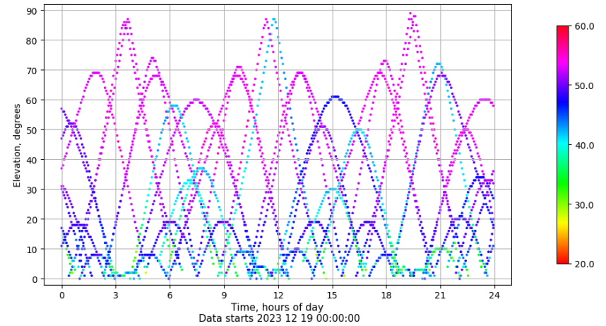
Time-elevation plot for station LEON. Signal to Noise S1C Data file LEON00ESP_R_2023353.xtr
