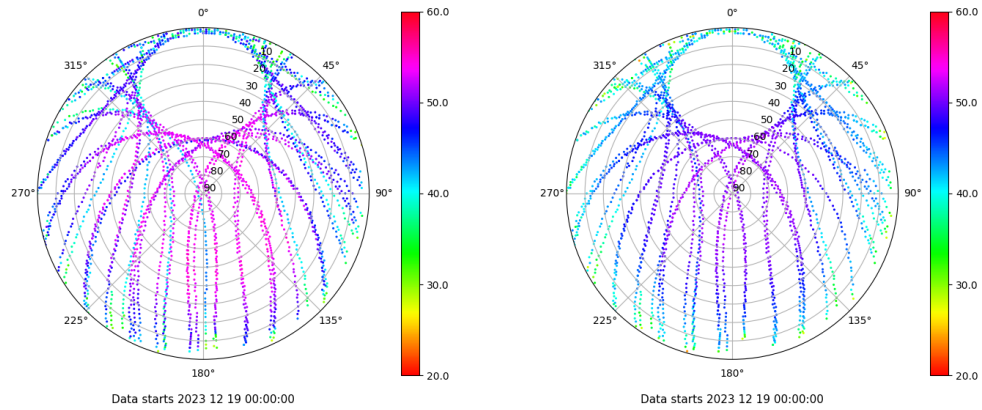
Skyplot for station LEON. Signal to Noise S1C Data file LEON00ESP_R_2023353.xtr Skyplot for station LEON. Signal to Noise S2P Data file LEON00ESP_R_2023353.xtr
