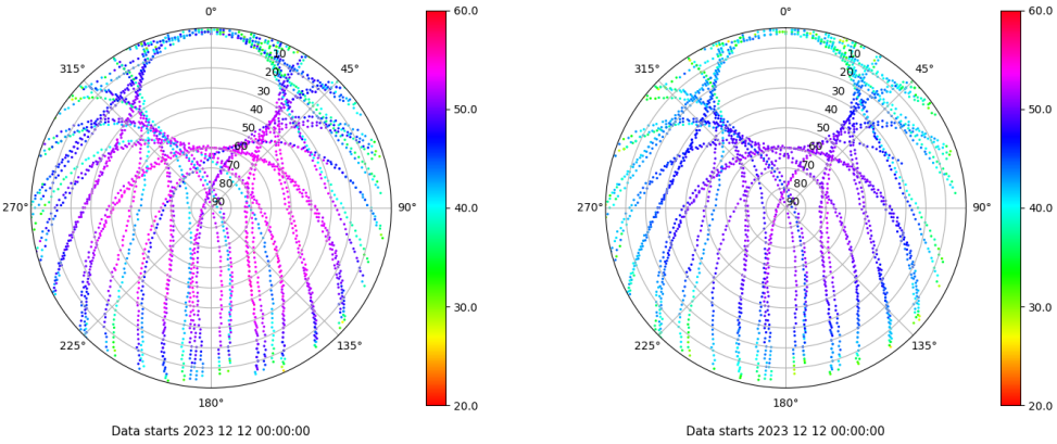
Skyplot for station LEON. Signal to Noise S1C Data file LEON00ESP_R_2023346.xtr Skyplot for station LEON. Signal to Noise S2P Data file LEON00ESP_R_2023346.xtr
