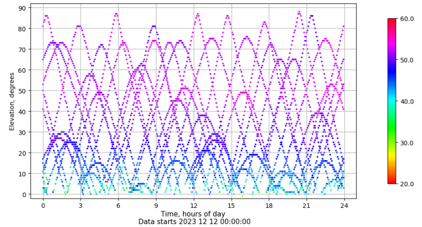
Time-elevation plot for station LEON. Signal to Noise S1C Data file LEON00ESP_R_2023346.xtr
