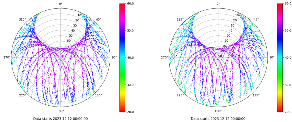
Skyplot for station LEON. Signal to Noise S1C Data file LEON00ESP_R_2023346.xtr Skyplot for station LEON. Signal to Noise S2W Data file LEON00ESP_R_2023346.xtr
