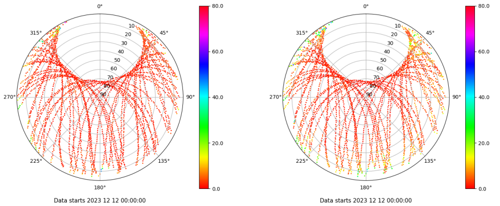
Skyplot for station LEON. Parameter M1C Data file LEON00ESP_R_2023346.xtr Skyplot for station LEON. Parameter M2W Data file LEON00ESP_R_2023346.xtr
