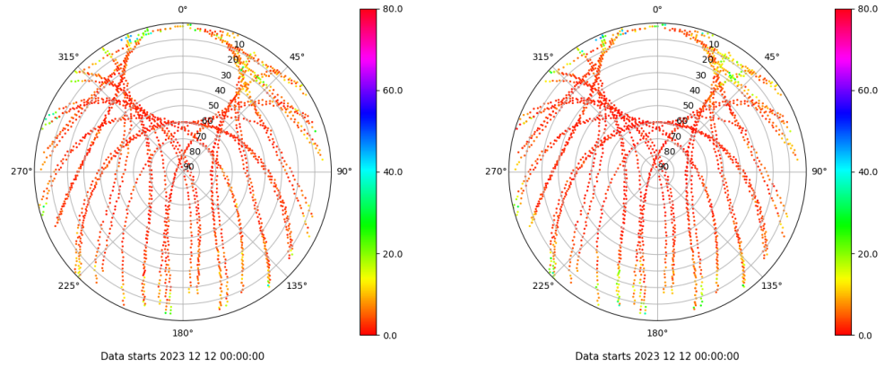
Skyplot for station LEON. Parameter M1C Data file LEON00ESP_R_2023346.xtr Skyplot for station LEON. Parameter M2P Data file LEON00ESP_R_2023346.xtr
