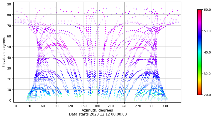
Azimuth-elevation plot for station LEON. Signal to Noise S1C Data file LEON00ESP_R_2023346.xtr
