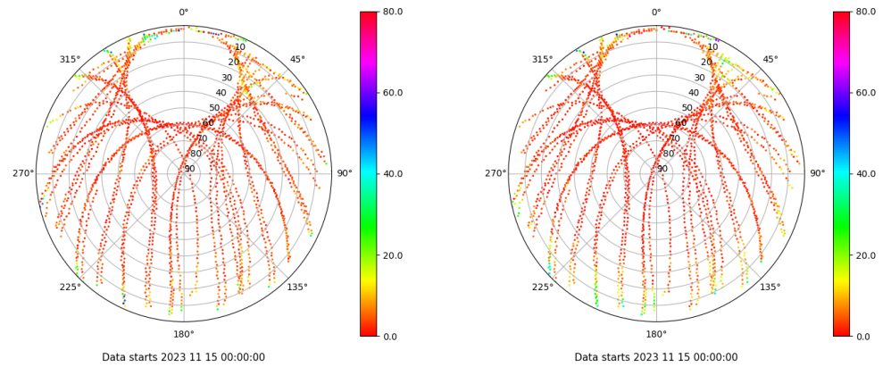
Skyplot for station LEON. Parameter M1C Data file LEON00ESP_R_2023319.xtr Skyplot for station LEON. Parameter M2P Data file LEON00ESP_R_2023319.xtr
