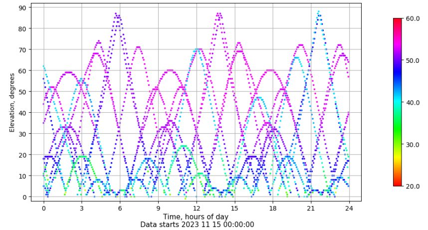
Time-elevation plot for station LEON. Signal to Noise S1C Data file LEON00ESP_R_2023319.xtr
