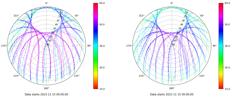
Skyplot for station LEON. Signal to Noise S1C Data file LEON00ESP_R_2023319.xtr Skyplot for station LEON. Signal to Noise S2P Data file LEON00ESP_R_2023319.xtr
