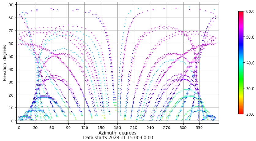
Azimuth-elevation plot for station LEON. Signal to Noise S1C Data file LEON00ESP_R_2023319.xtr
