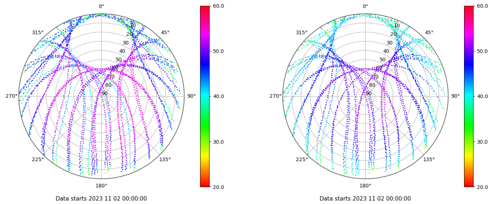
Skyplot for station LEON. Signal to Noise S1C Data file LEON00ESP_R_2023306.xtr Skyplot for station LEON. Signal to Noise S2P Data file LEON00ESP_R_2023306.xtr
