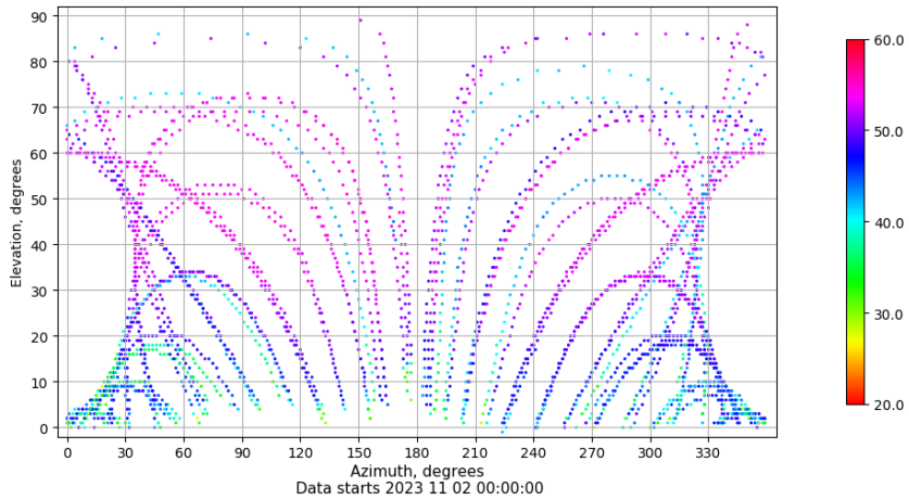
Azimuth-elevation plot for station LEON. Signal to Noise S1C Data file LEON00ESP_R_2023306.xtr
