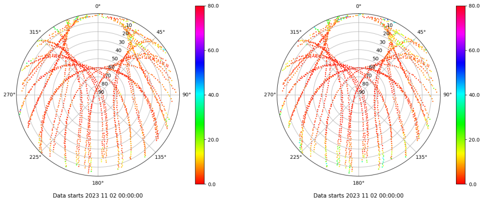
Skyplot for station LEON. Parameter M1C Data file LEON00ESP_R_2023306.xtr Skyplot for station LEON. Parameter M2P Data file LEON00ESP_R_2023306.xtr
