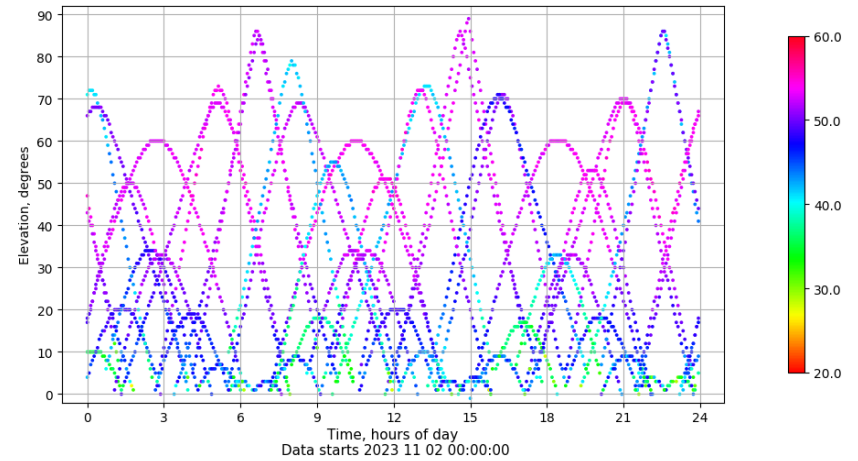
Time-elevation plot for station LEON. Signal to Noise S1C Data file LEON00ESP_R_2023306.xtr
