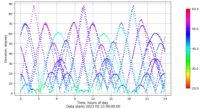
Time-elevation plot for station LEON. Signal to Noise S1C Data file LEON00ESP_R_2023133.xtr
