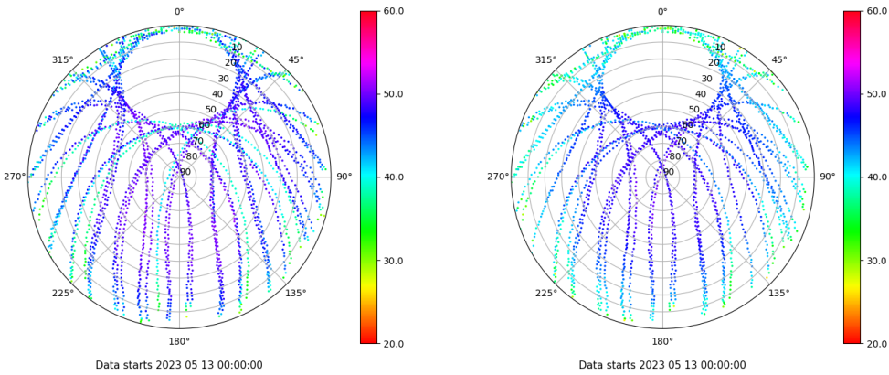
Skyplot for station LEON. Signal to Noise S1C Data file LEON00ESP_R_2023133.xtr Skyplot for station LEON. Signal to Noise S2P Data file LEON00ESP_R_2023133.xtr
