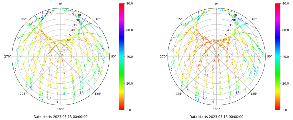
Skyplot for station LEON. Parameter M1C Data file LEON00ESP_R_2023133.xtr Skyplot for station LEON. Parameter M2P Data file LEON00ESP_R_2023133.xtr
