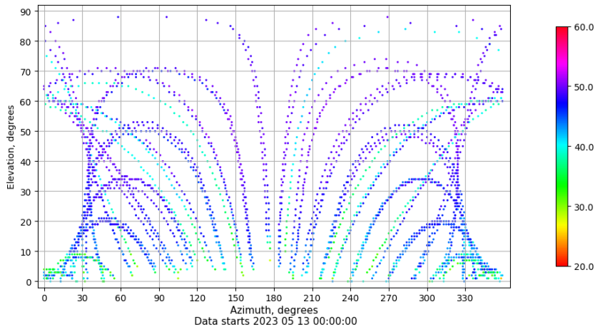
Azimuth-elevation plot for station LEON. Signal to Noise S1C Data file LEON00ESP_R_2023133.xtr
