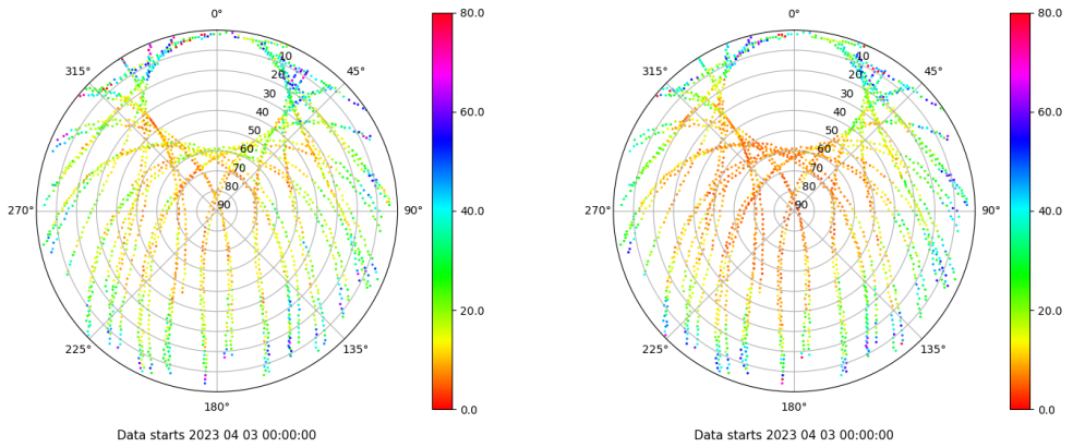
Skyplot for station LEON. Parameter M1C Data file LEON00ESP_R_2023093.xtr Skyplot for station LEON. Parameter M2P Data file LEON00ESP_R_2023093.xtr
