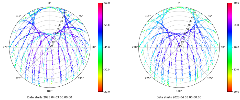
Skyplot for station LEON. Signal to Noise S1C Data file LEON00ESP_R_2023093.xtr Skyplot for station LEON. Signal to Noise S2P Data file LEON00ESP_R_2023093.xtr
