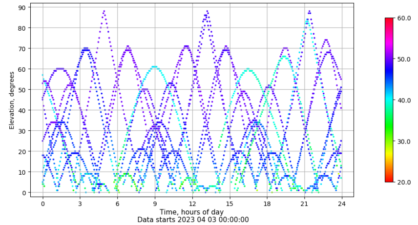
Time-elevation plot for station LEON. Signal to Noise S1C Data file LEON00ESP_R_2023093.xtr
