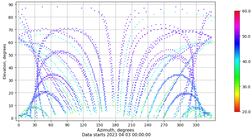
Azimuth-elevation plot for station LEON. Signal to Noise S1C Data file LEON00ESP_R_2023093.xtr
