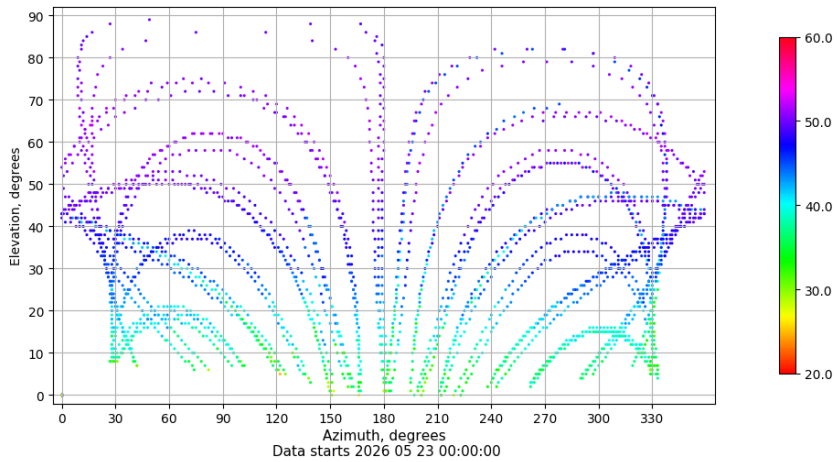
Azimuth-elevation plot for station LALA. Signal to Noise S1C Data file LALA00ESP_R_2026143.xtr
