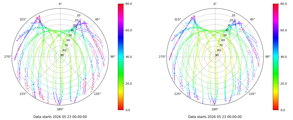
Skyplot for station LALA. Parameter M1C Data file LALA00ESP_R_2026143.xtr Skyplot for station LALA. Parameter M2C Data file LALA00ESP_R_2026143.xtr
