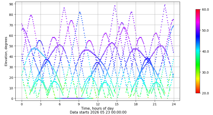
Time-elevation plot for station LALA. Signal to Noise S1C Data file LALA00ESP_R_2026143.xtr
