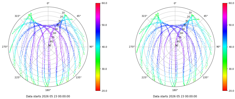
Skyplot for station LALA. Signal to Noise S1C Data file LALA00ESP_R_2026143.xtr Skyplot for station LALA. Signal to Noise S2C Data file LALA00ESP_R_2026143.xtr
